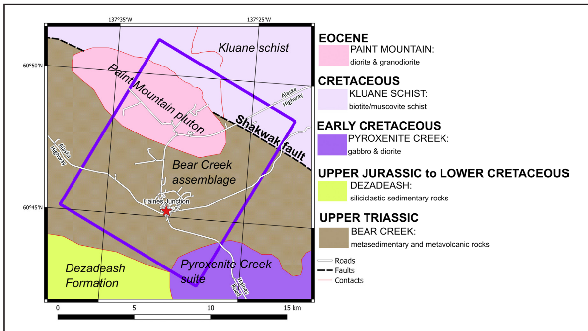
Figure 3. Bedrock geology in the Haines Junction area, Yukon (adapted from Colpron, 2022 and Yukon Geological Survey, 2023b). The study area is delineated by the purple rectangle.
