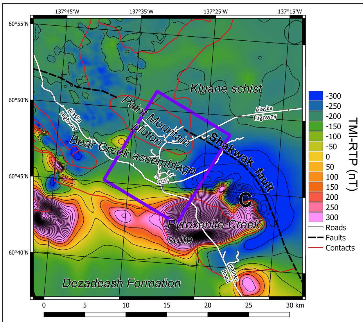
Figure 5. Magnetic survey data for the greater Haines Junction area plotted as Total Magnetic Intensity-Reduced to Pole (TMI-RTP). The data are gridded with a 100 m cell size and coloured with cool/warm colours representing magnetic lows/highs. See text for discussion.
