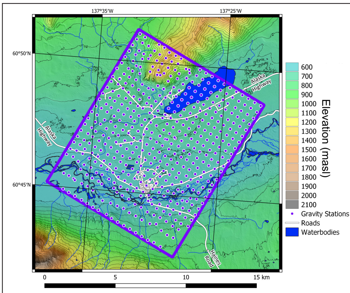
Figure 6. Map showing gravity stations (purple dots) from the 2022/2023 gravity survey by Aurora Geosciences. The survey area is ~10 km by ~12.5 km (purple rectangle). The background image shows topography, waterbodies and roads.
