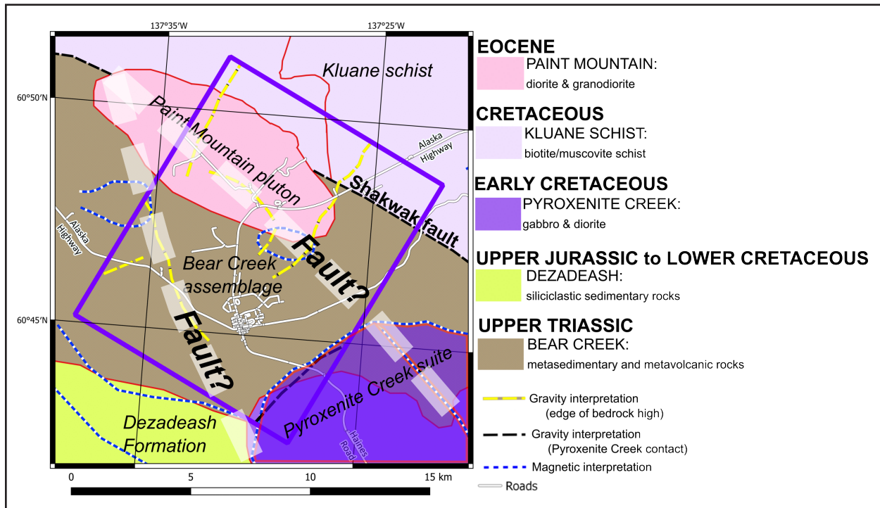
Figure 13. Map-based structural interpretation for the Haines Junction area derived from co-interpretation of gravity, magnetic and bedrock geology data. Large dashed white lines are proposed fault structures that are interpreted as splays of the Shakwak fault. See text for discussion.
