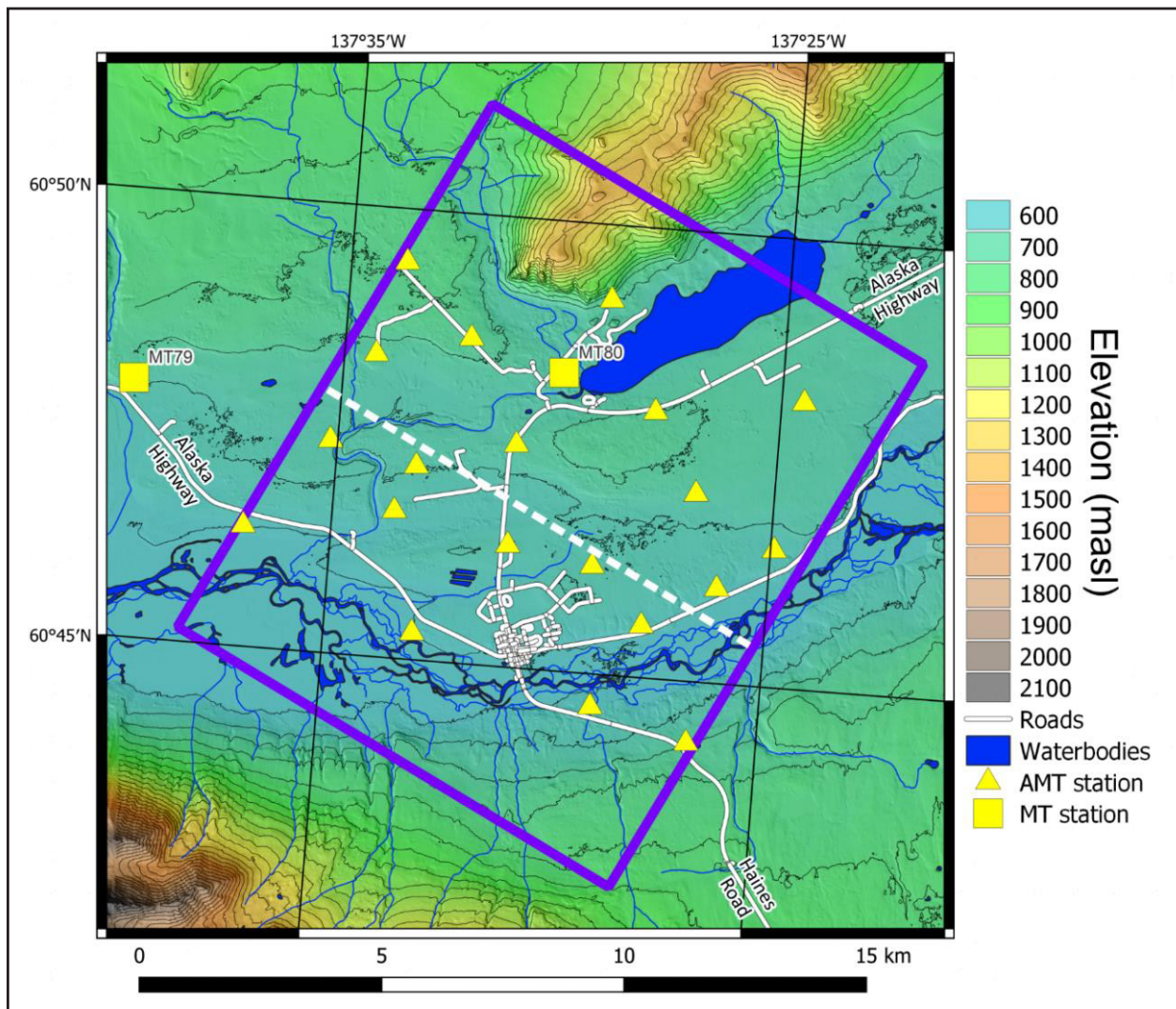
Figure 7. Map showing locations of AMT (yellow triangles) and MT (yellow squares) stations used by Geological Survey of Canada to generate the 3D resistivity inversion model. Location of resistivity cross-section (Fig. 14) is shown by the white dashed line.
