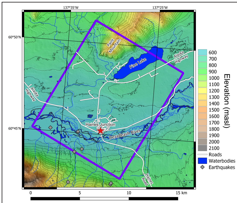
Figure 2. Location map showing the ~10 km by ~12.5 km study area (purple box). Historic earthquake epicentres are also shown (grey diamonds). Contour interval is 50 m.
