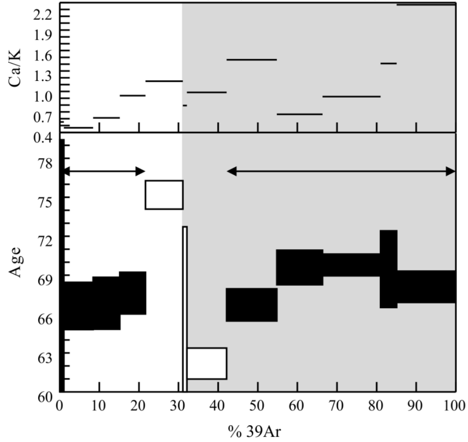
(A) Z4609 96CH-MN1 (WR) 68.5 \pm 1.2 Ma (MSWD=3.8)
