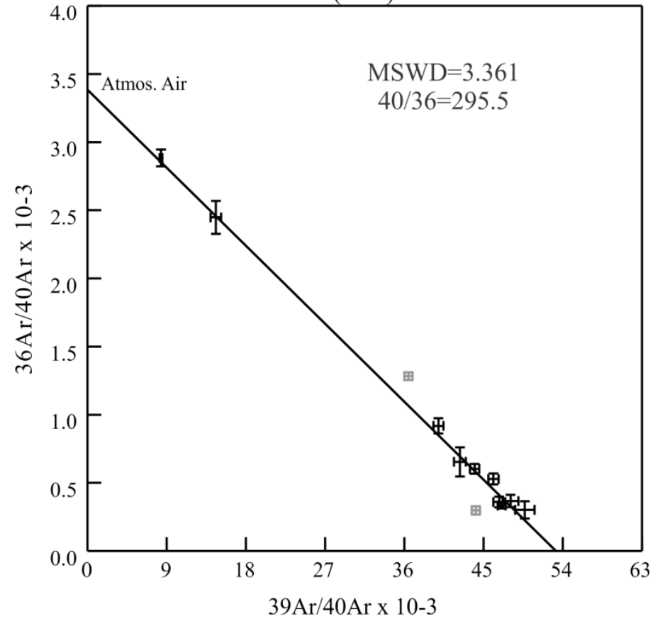
(B) Z4609 96CH-MN1 (WR) 68.5 \pm 1.1 Ma
