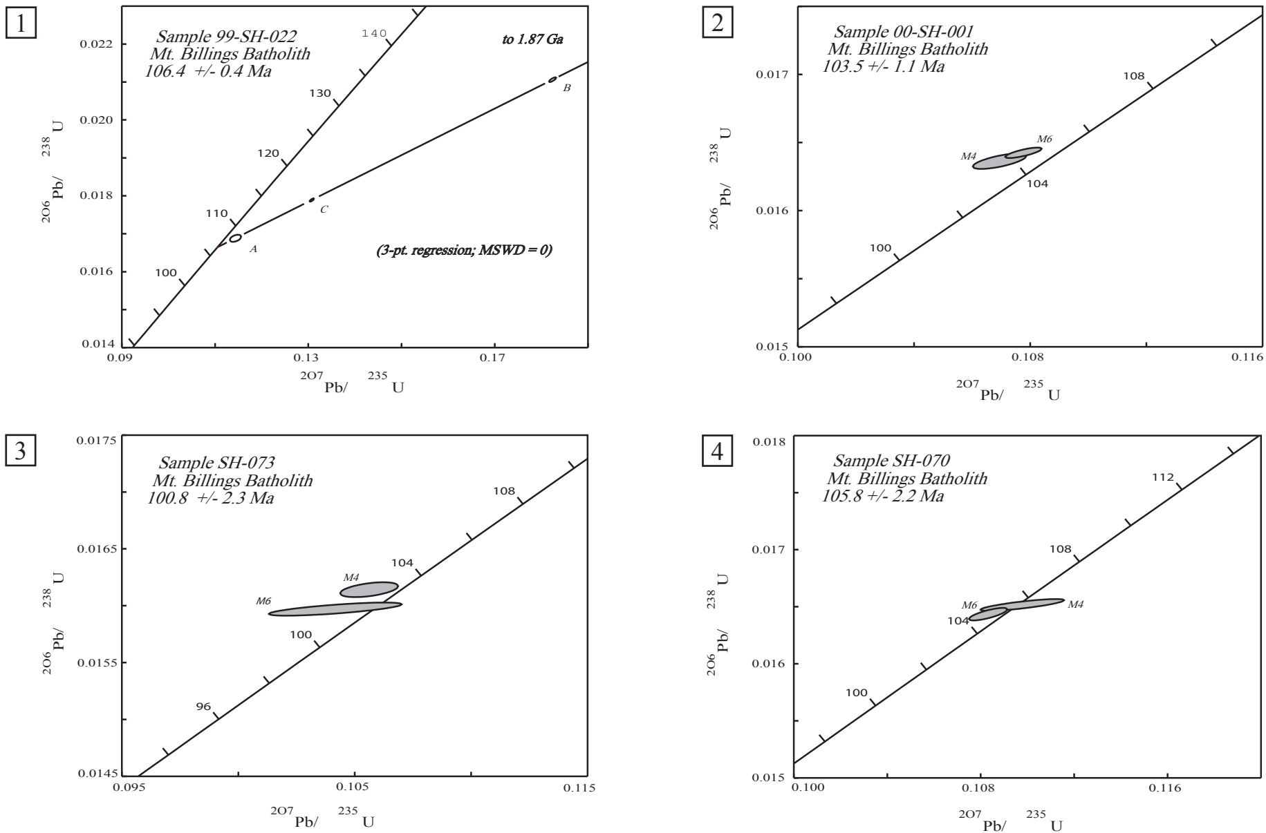
Figure 2.4. U-Pb concordia plots for intrusions from southeast Yukon and southwest Northwest Territories used in this study. Open, shaded, and striped ellipses denote zircon, monazite, and titanite fractions, respectively. Results and interpretations are discussed in text.
