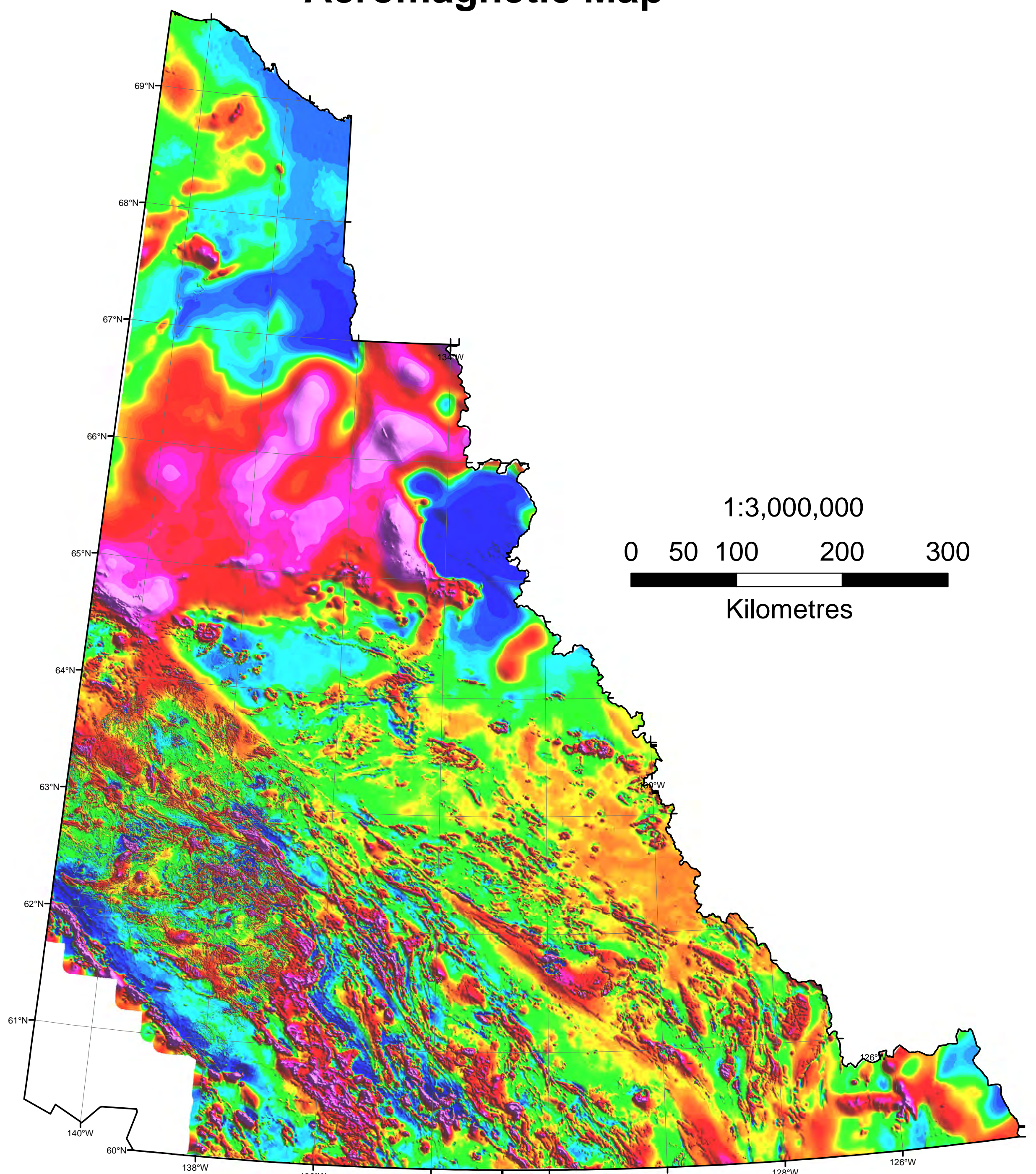
Aeromagnetic Map
