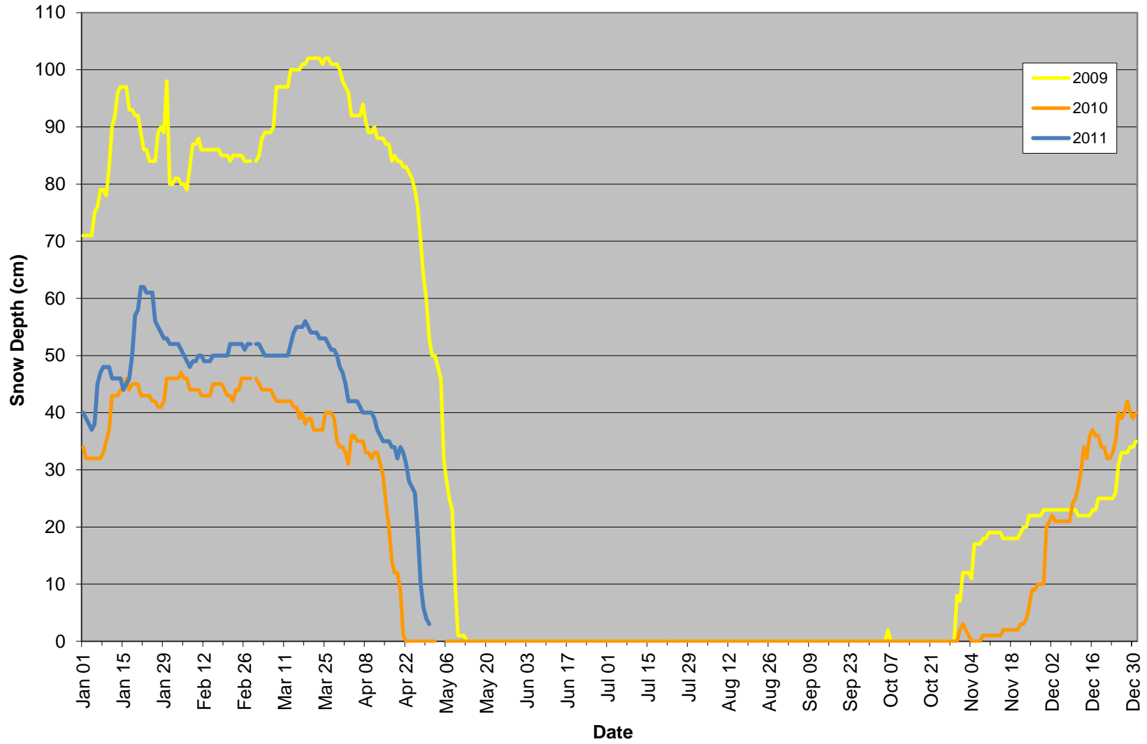
Watson Lake, Snow on Ground, 2009-2011 (data from Environment Canada "Watson Lake A" station)
