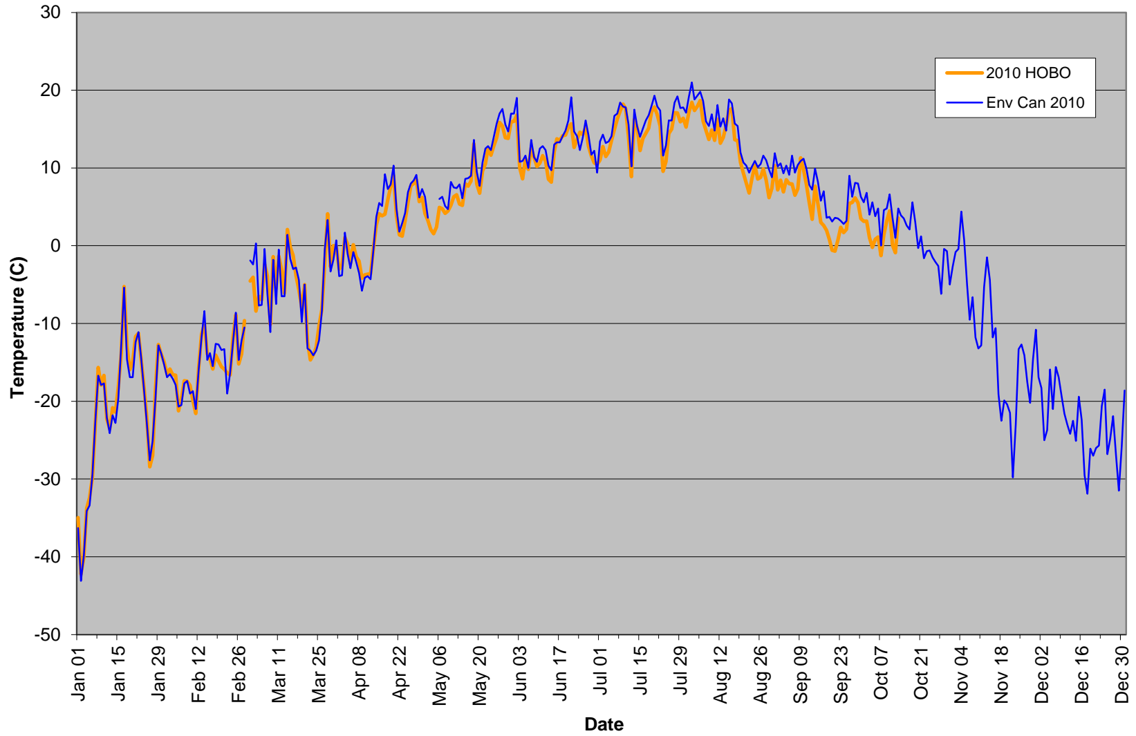
Watson Lake Average Daily Air Temperatures, 2010
