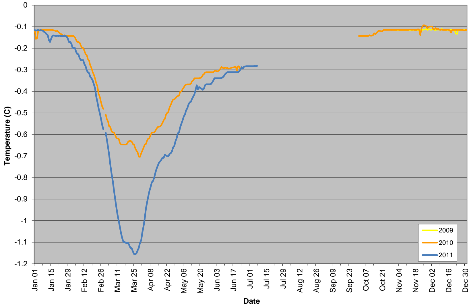
Watson Lake Average Daily Ground Temperatures at 1 m, 2009-2011
