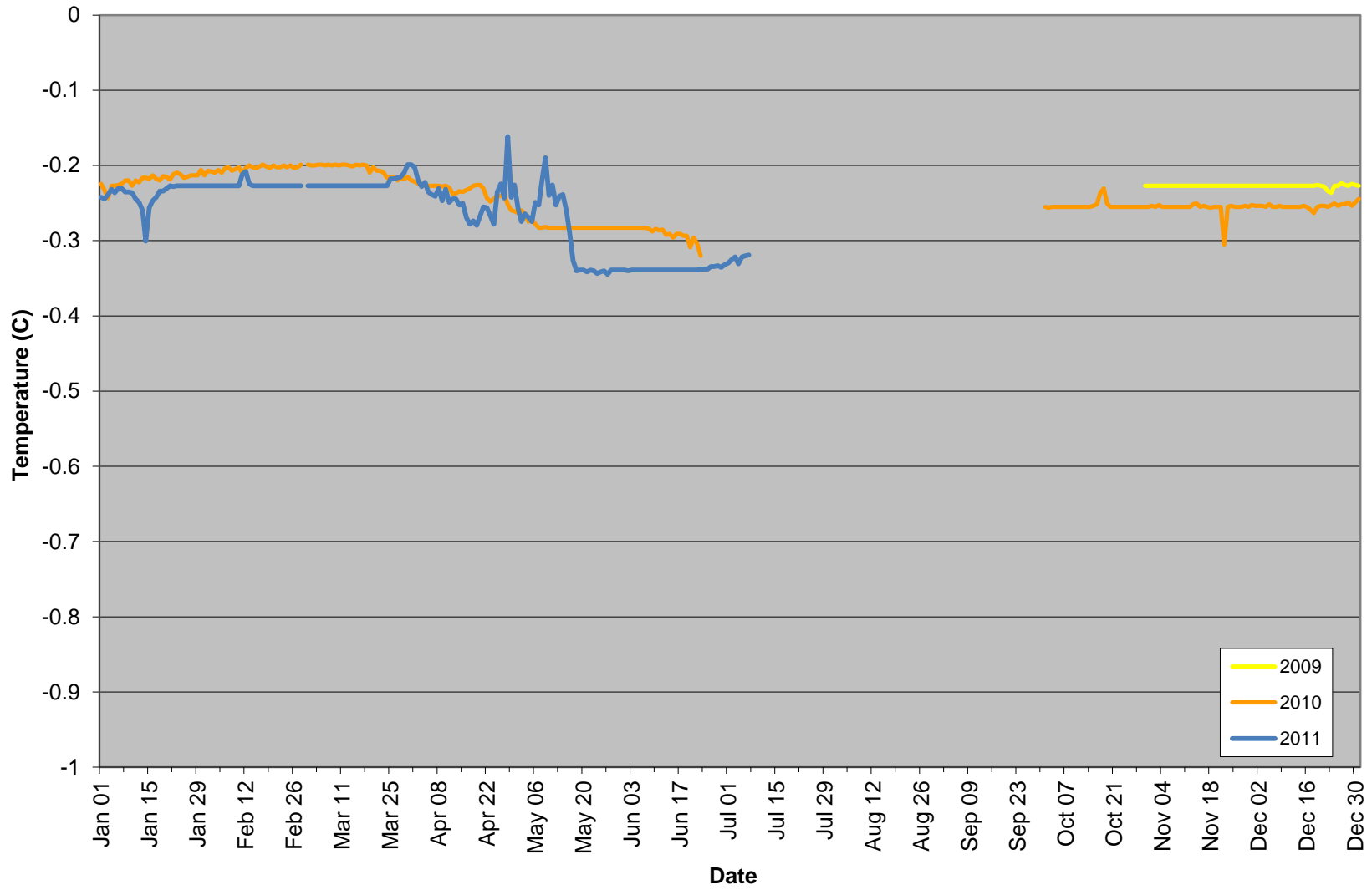
Watson Lake Average Daily Ground Temperatures at 2 m, 2009-2011
