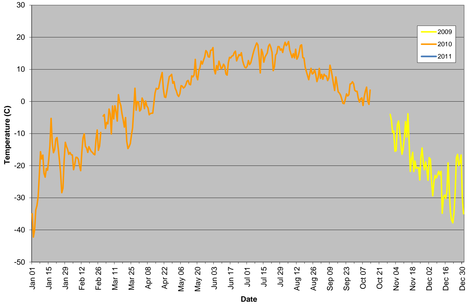
Watson Lake Average Daily Air Temperatures, 2009-2011
