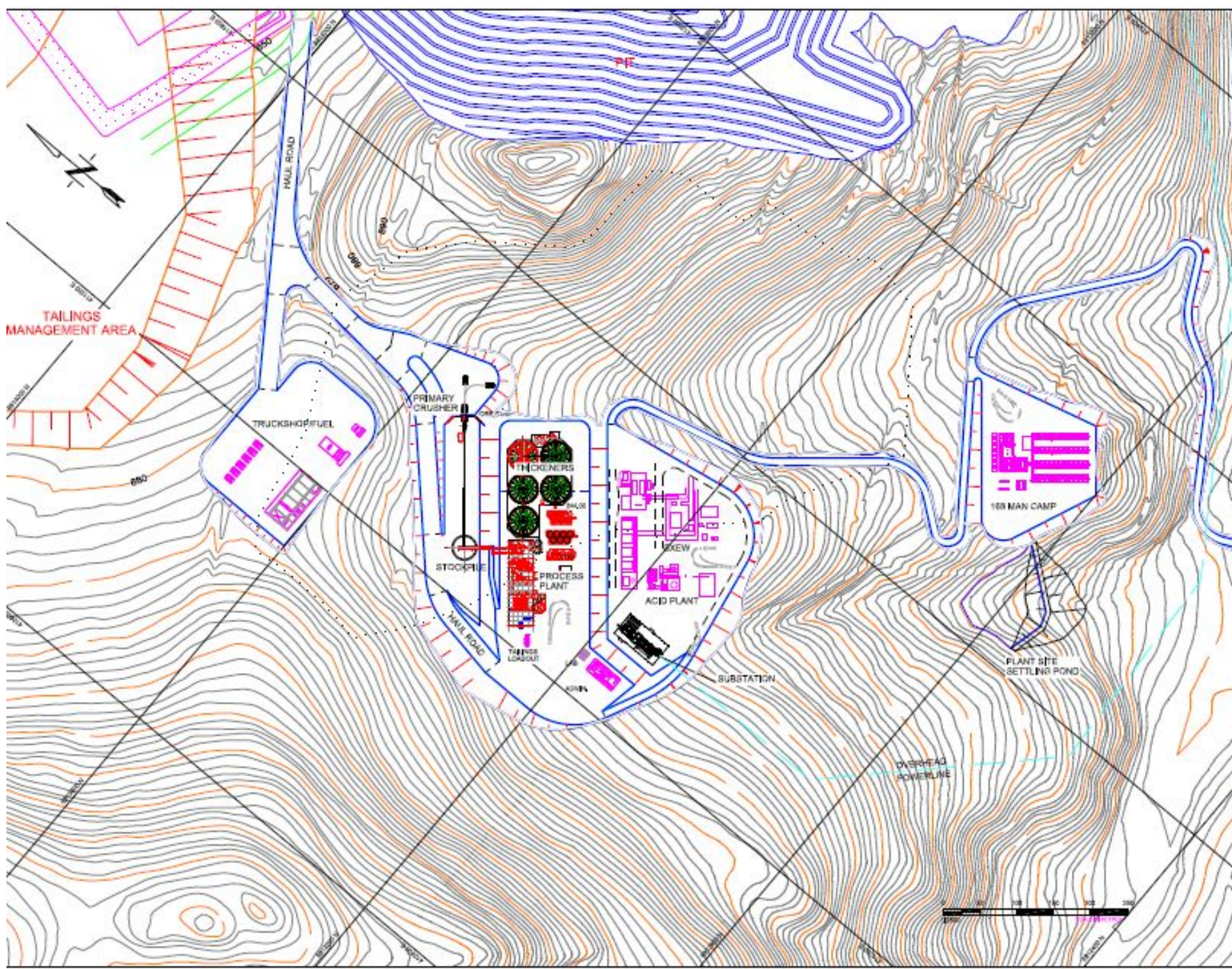
Figure 18.2: Plant Site Layout
