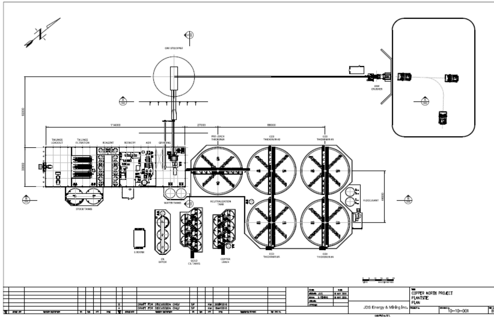
Figure 17.2: Process Plant Facilities
