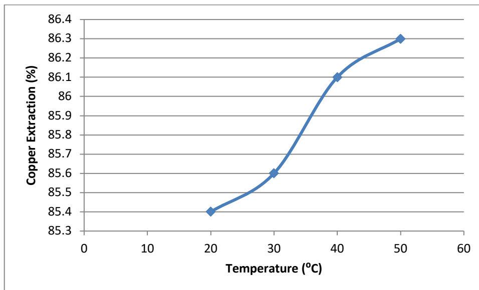
Figure 13.1: Slurry Temperature vs Copper Leach Extraction Rate
