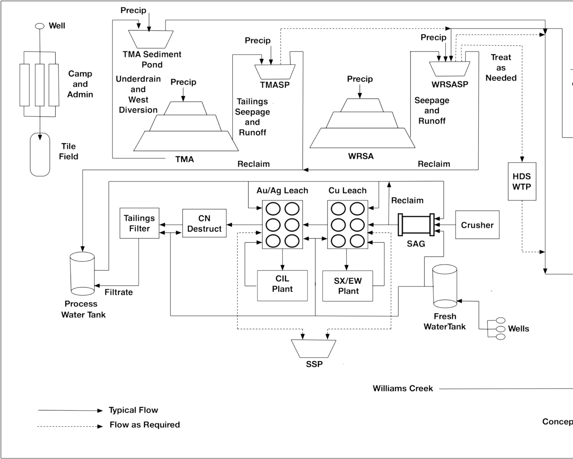
Figure 20.2: Conceptual Water Management Plan
