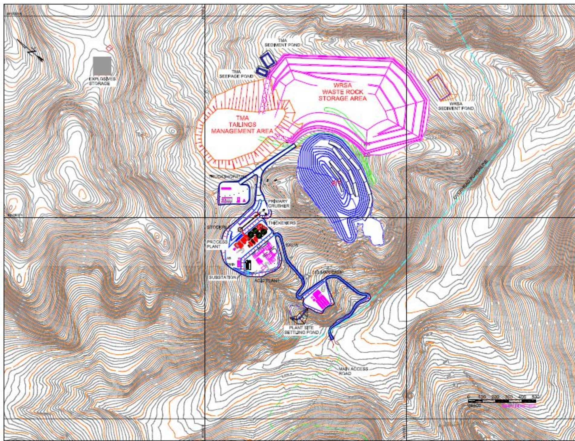
Figure 18.1: General Site Layout
