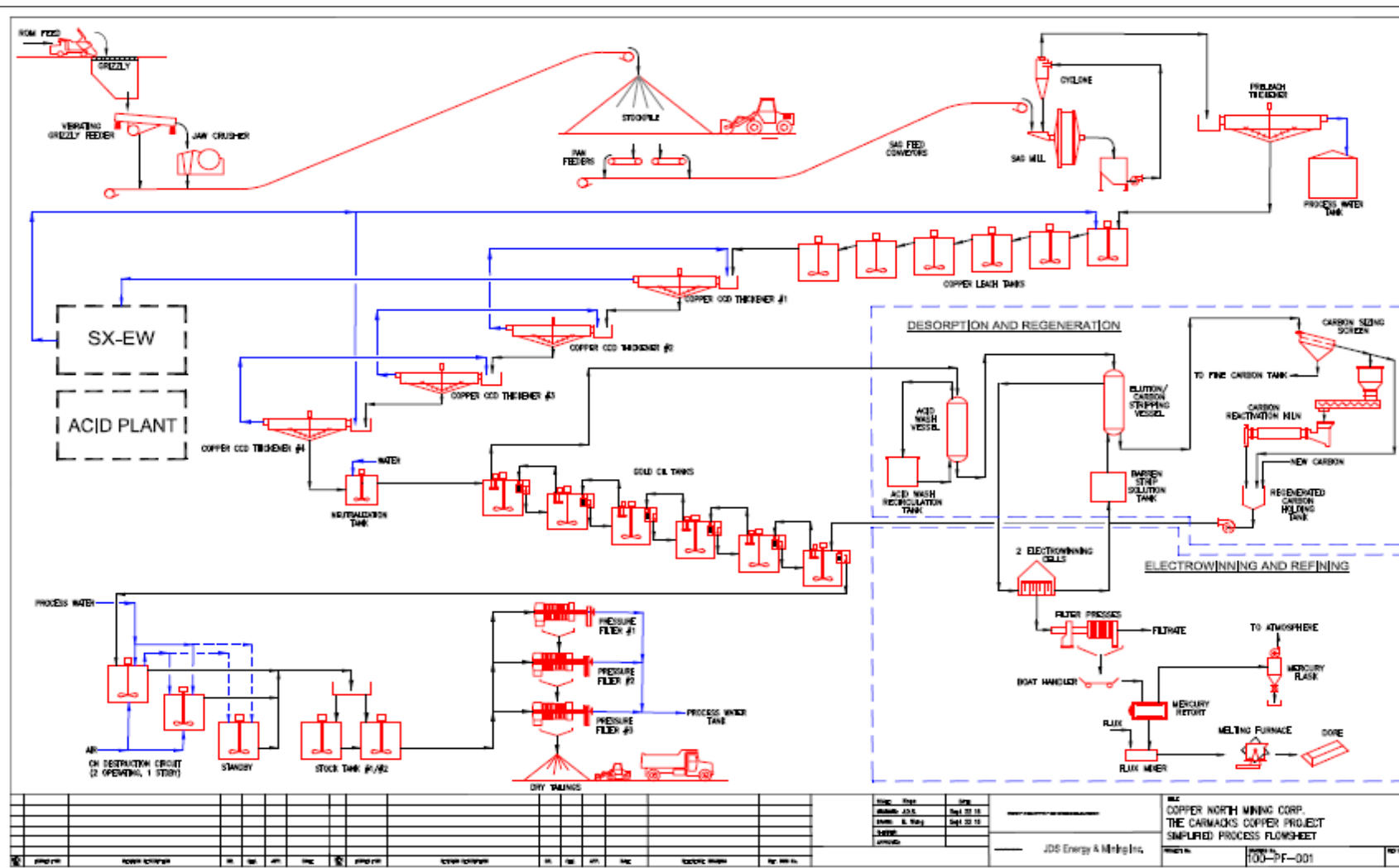
Figure 17.1: Overall Flowsheet
