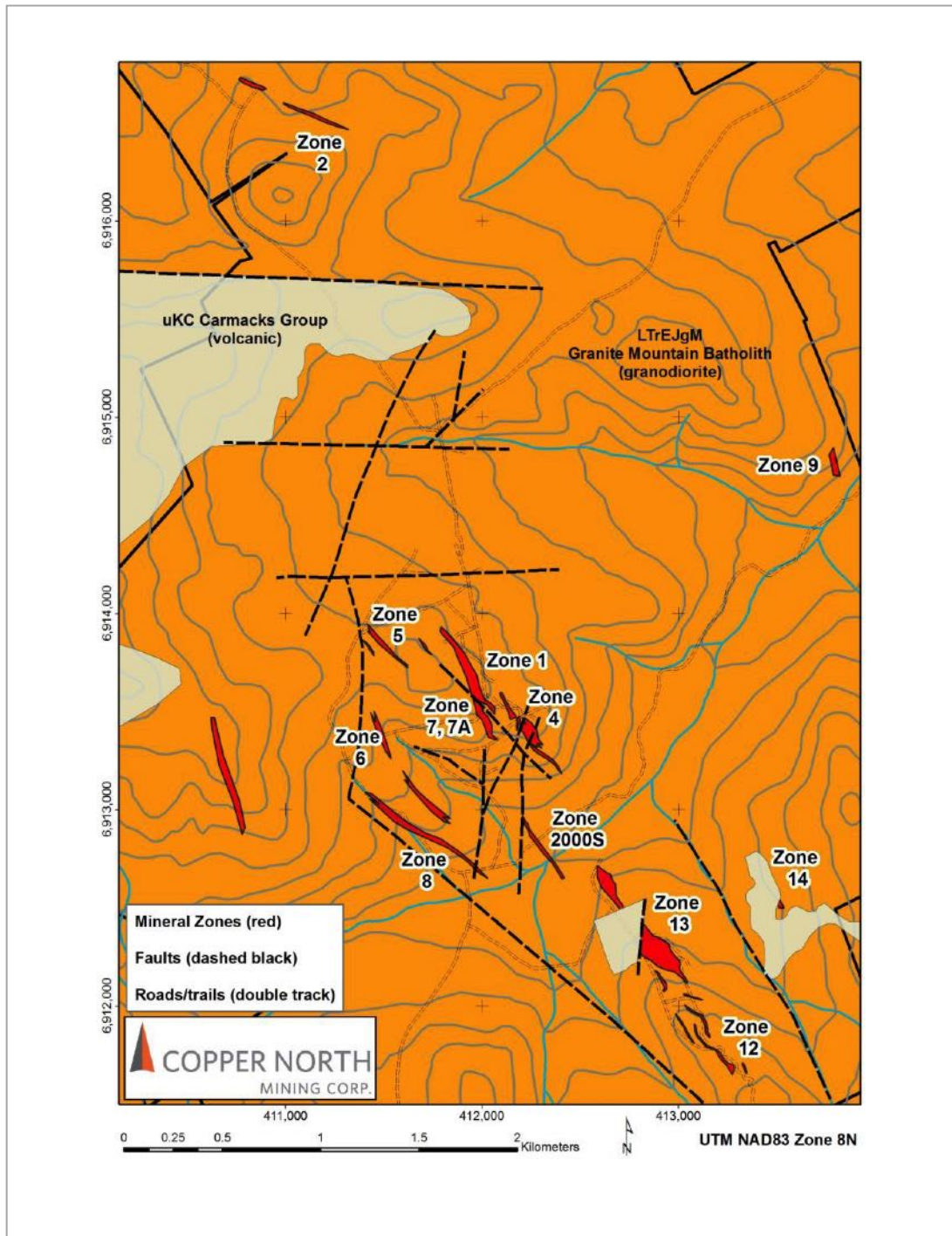
Figure 7.2: Property Geologic Map
