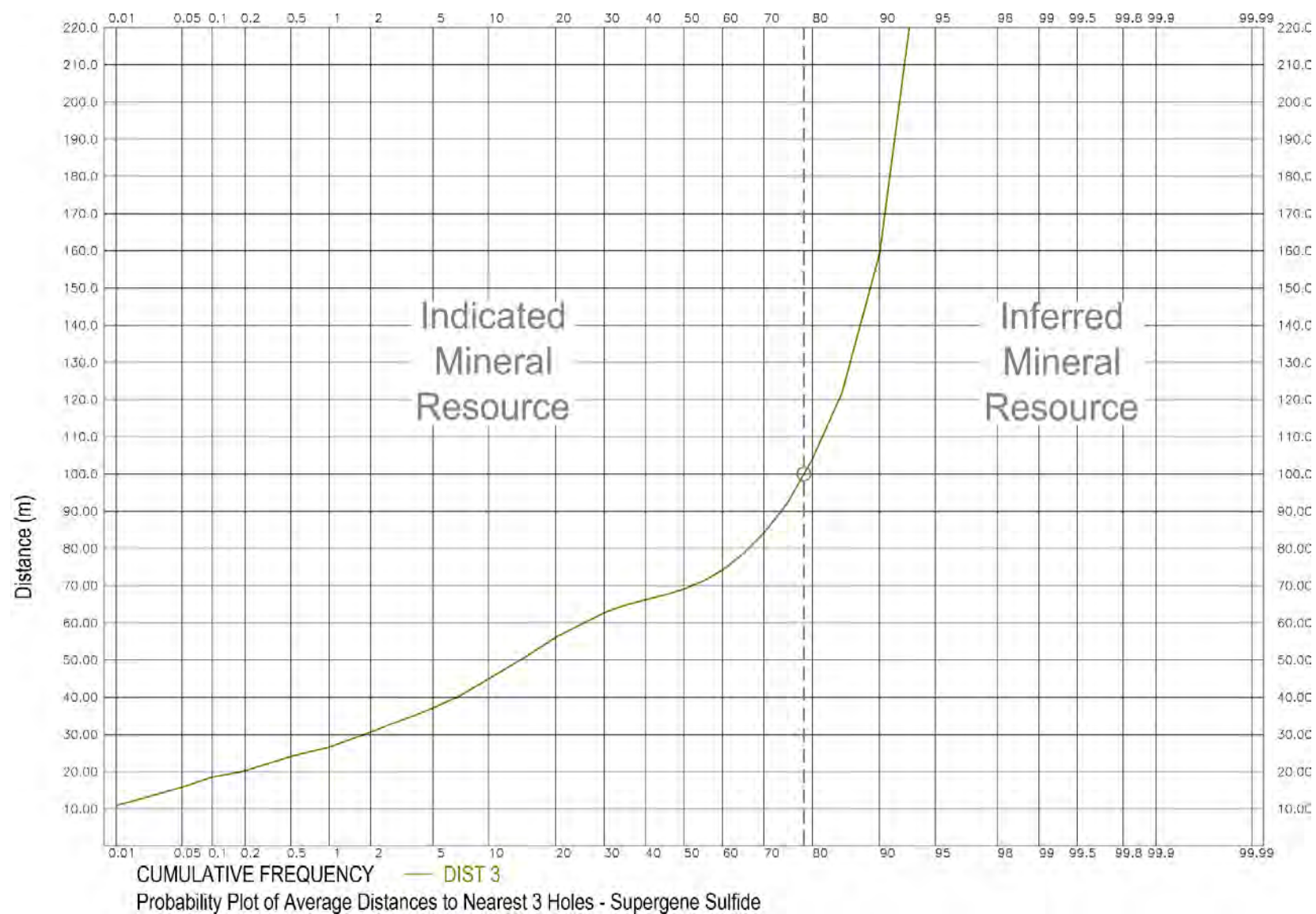
Figure 14-18: Probability Plot of Average Distance to Nearest 3 Holes – Supergene Sulphide (Source: IMC, 2020)
