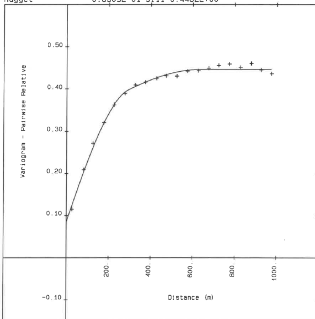
Figure 14-10: Total Copper Variogram – Hypogene Sulphide - Global
