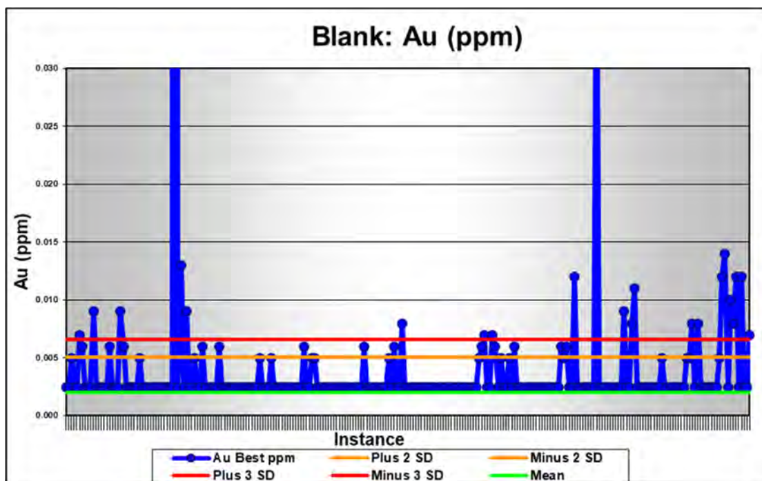
Figure 11-29: Gold assay results, blank material
