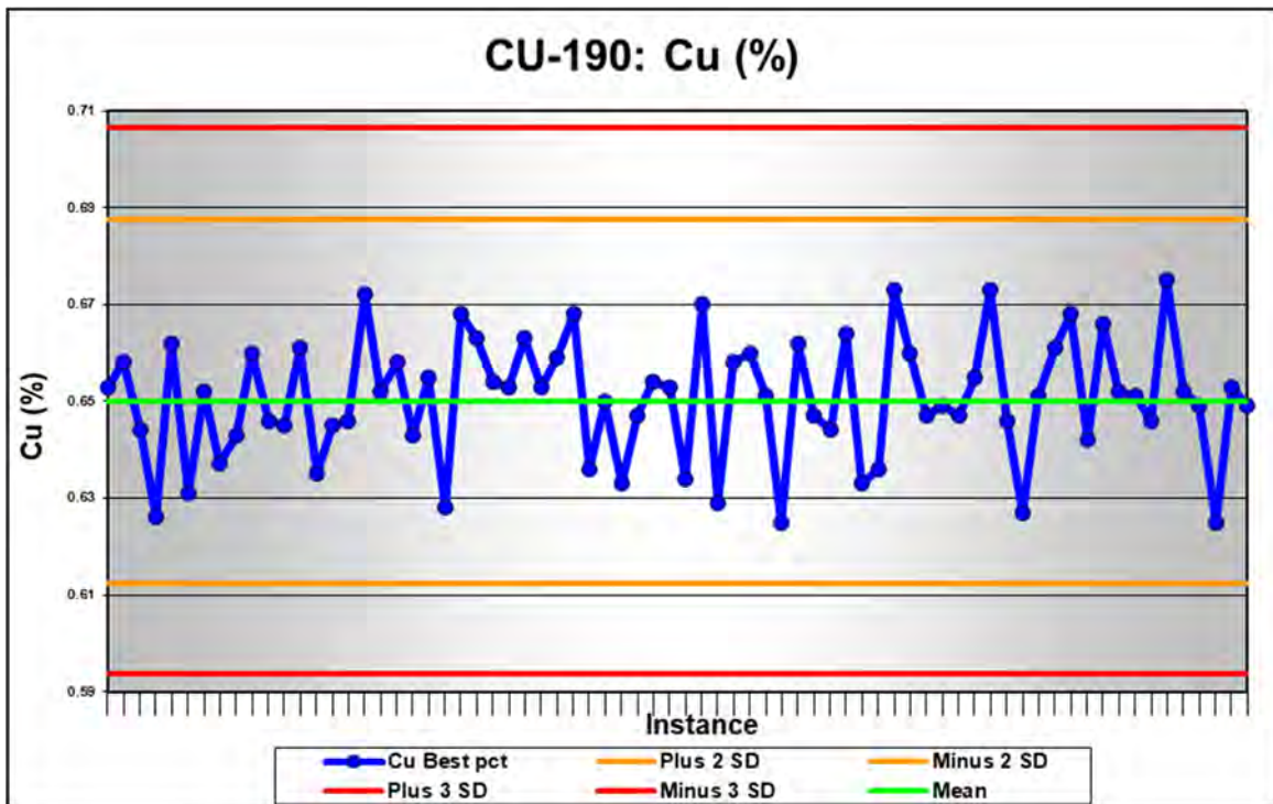
Figure 11-23: Standard CU-190 copper assay results
