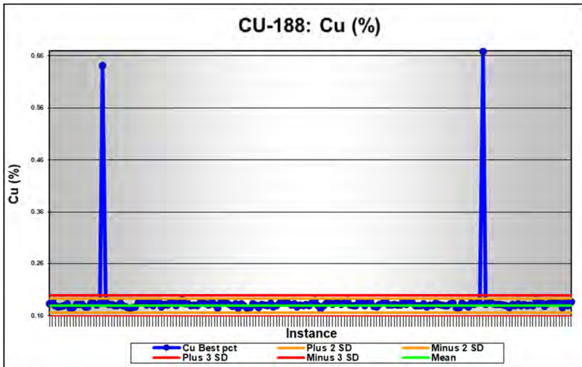
Figure 11-19: Standard Cu-188 copper assay results
