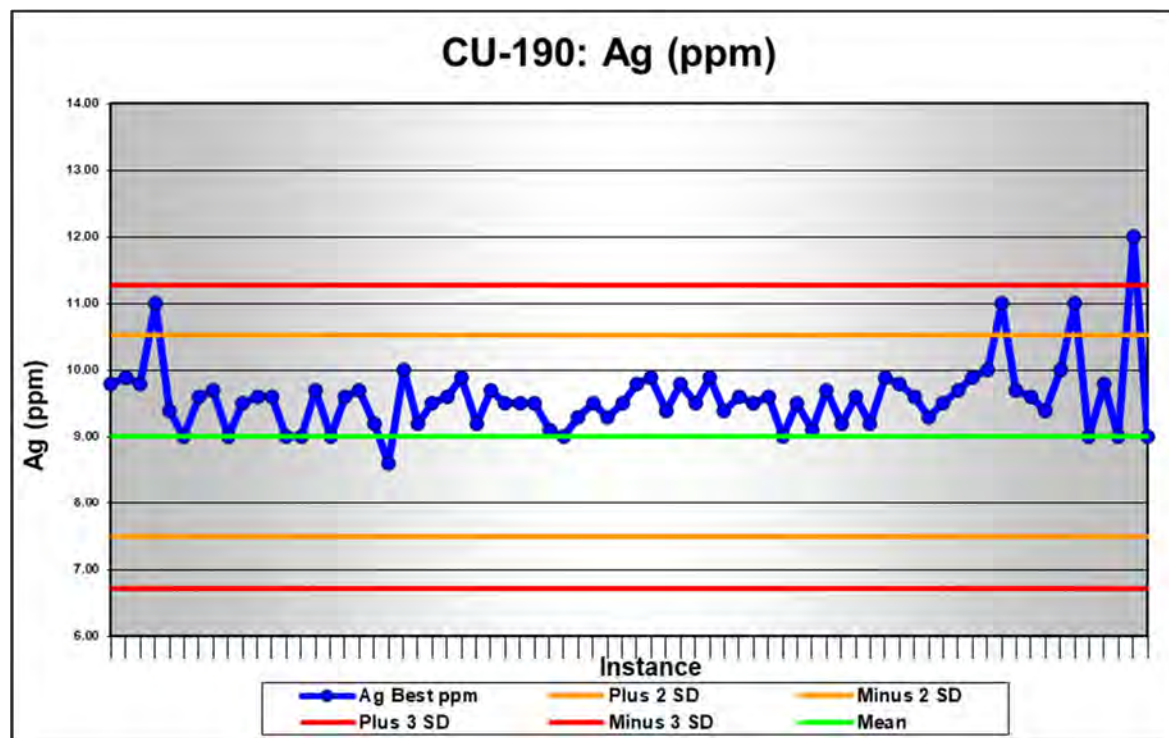
Figure 11-22: Standard Cu-190 silver assay results
