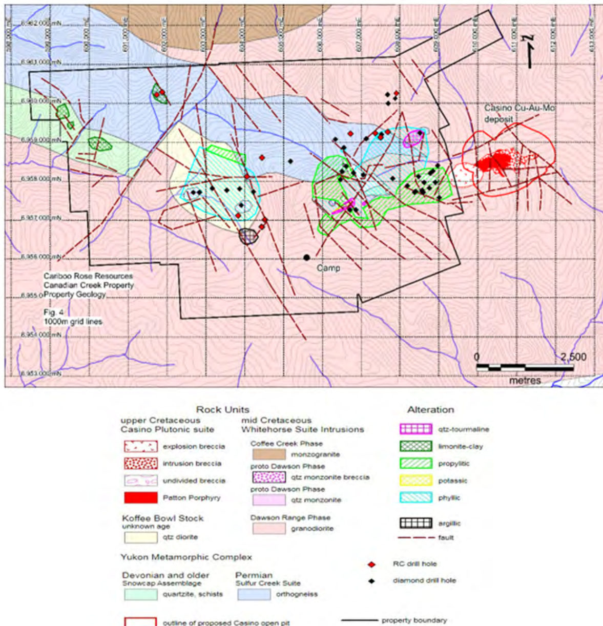
Figure 7-3: Property Geology (From R. Johnston, 2018)
