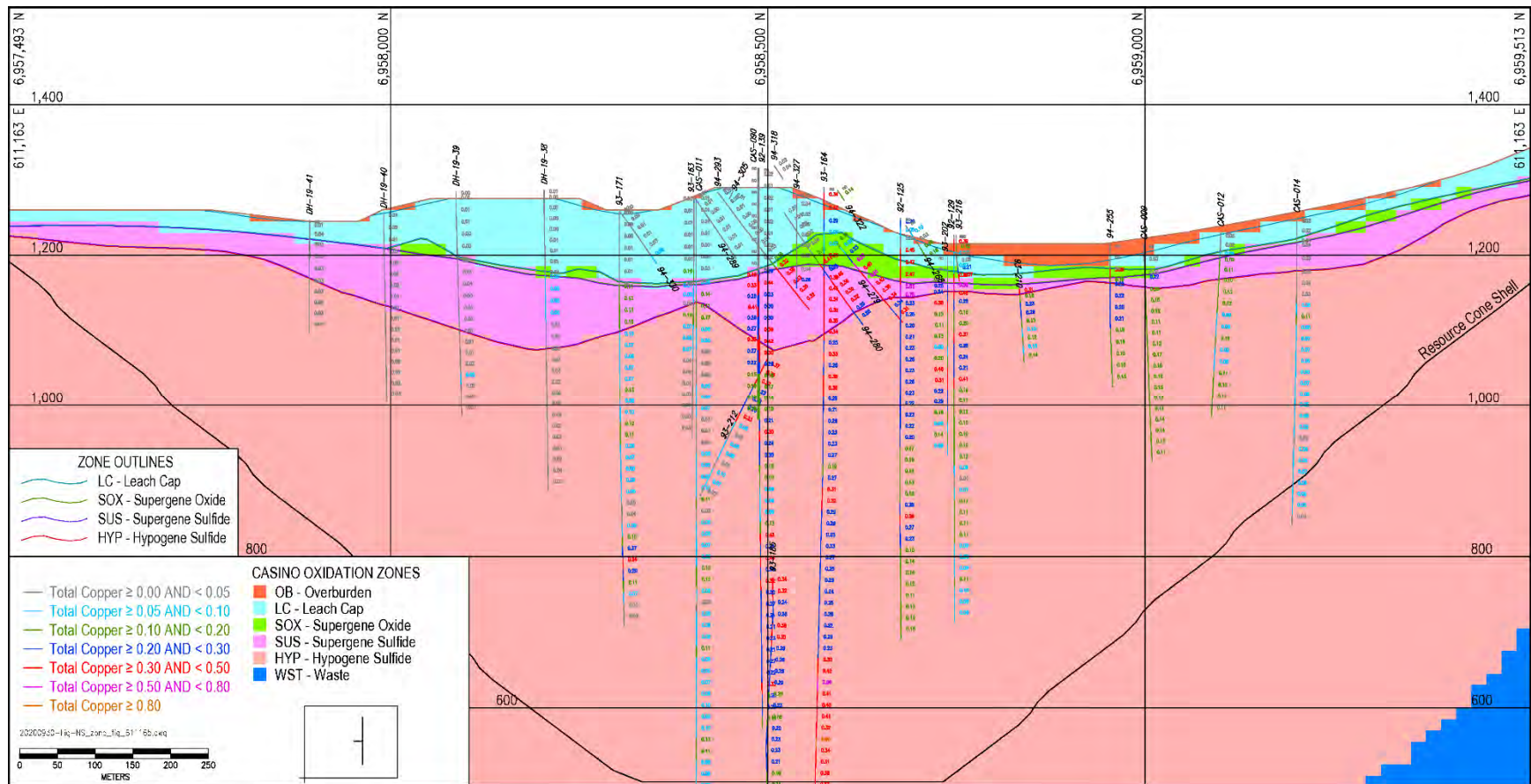
Figure 14-4: Oxidation Domains on North-South Section 611,165E
