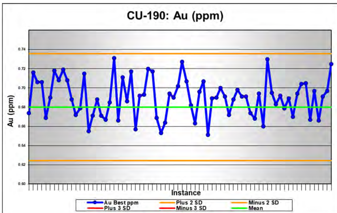
Figure 11-21: Standard Cu-190 gold assay results
