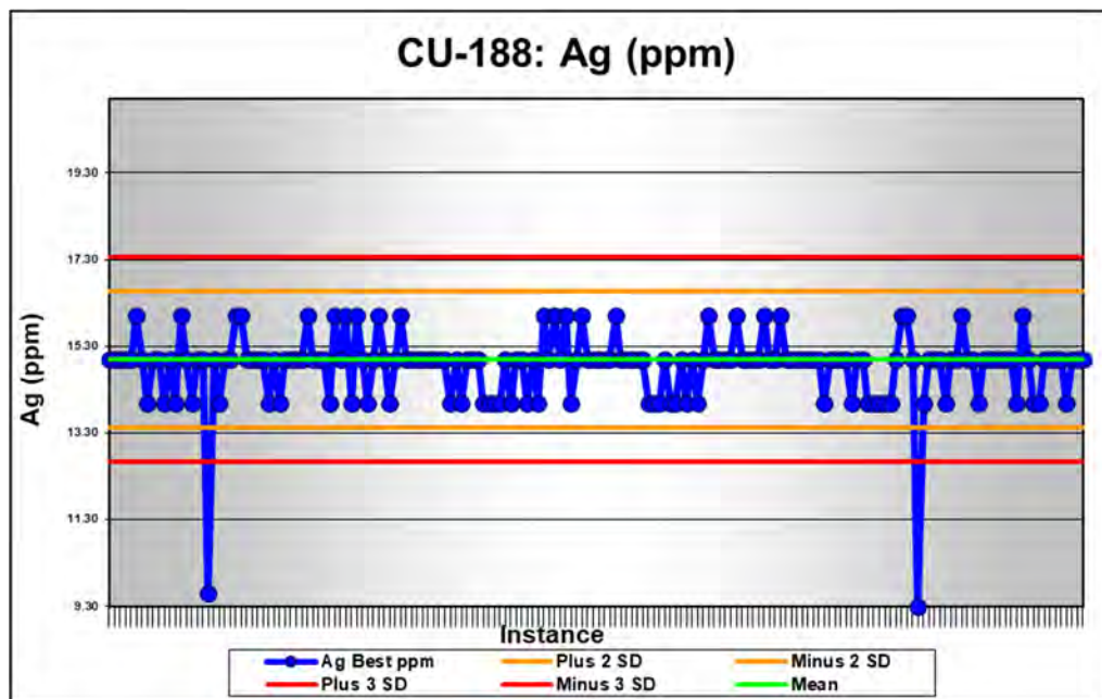
Figure 11-18: Standard Cu-188 silver assay results
