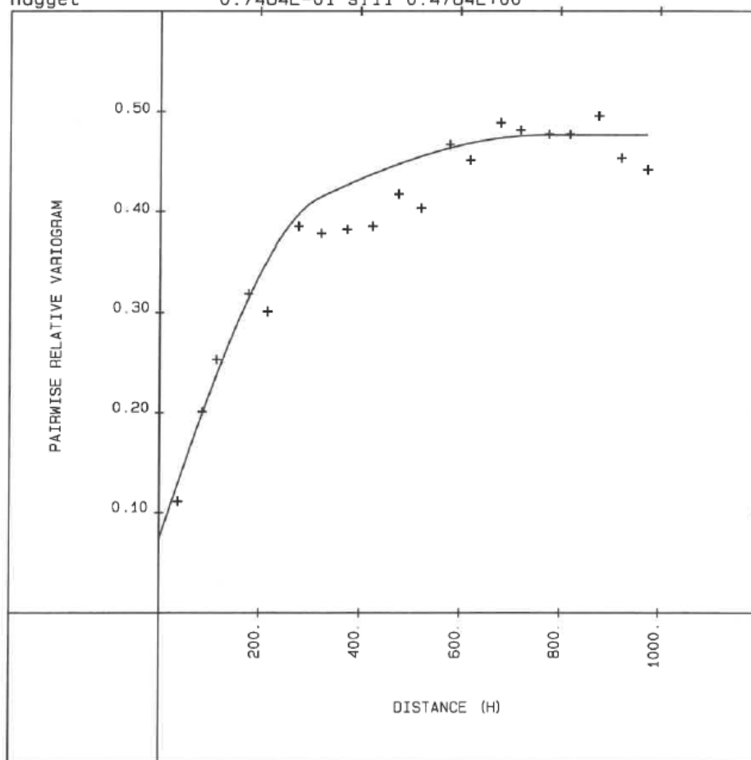
Figure 14-11: Total Copper Variogram – Hypogene Sulphide – East-West
