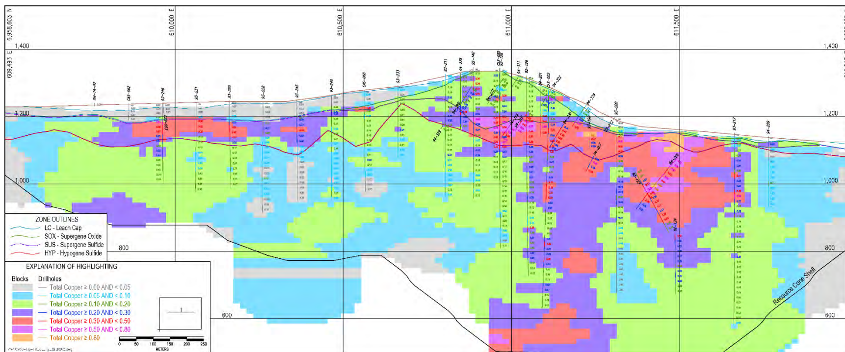
Figure 14-14: Total Copper Grades on East-West Cross Section 6,958,600N
