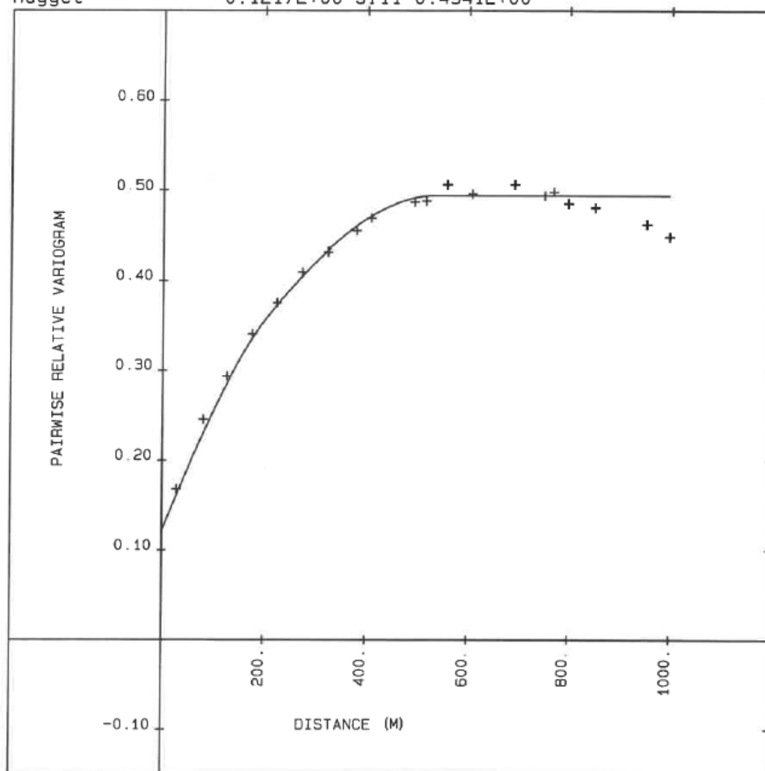
Figure 14-13: Gold Variogram
