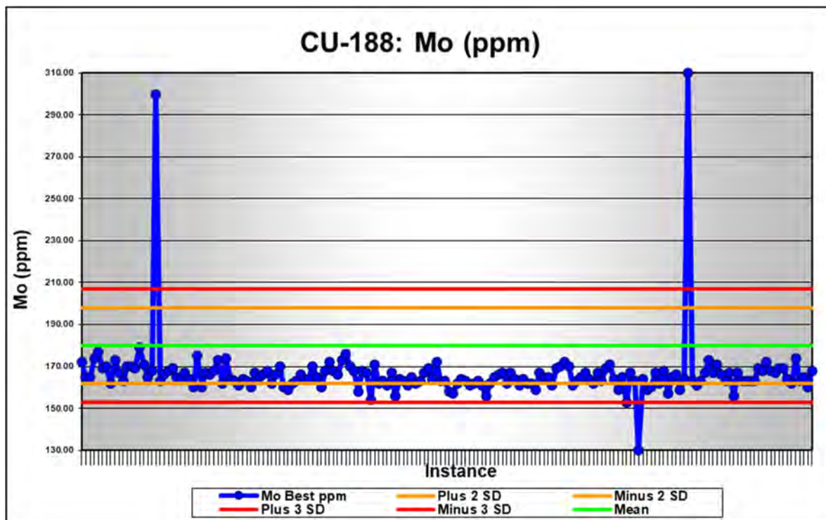
Figure 11-20: Standard Cu-188 molybdenum assay results
