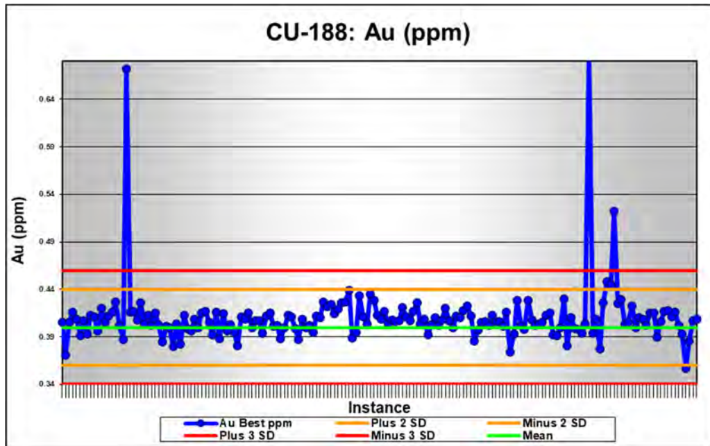
Figure 11-17: Standard CU-188 gold assay results
