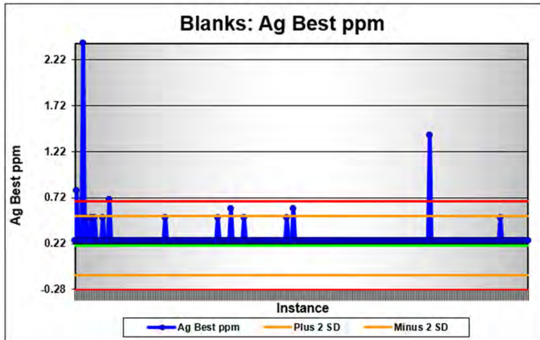
Figure 11-26: Blank Material Silver Assay Results
