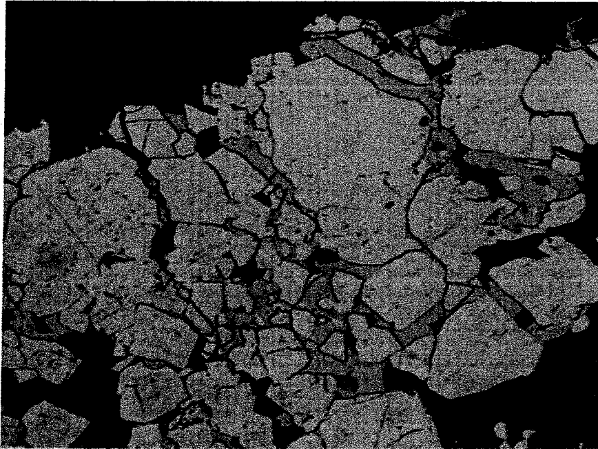
Photo 1. Fyre Lake Deposit PS6506 Mag 100X Reflected Light
