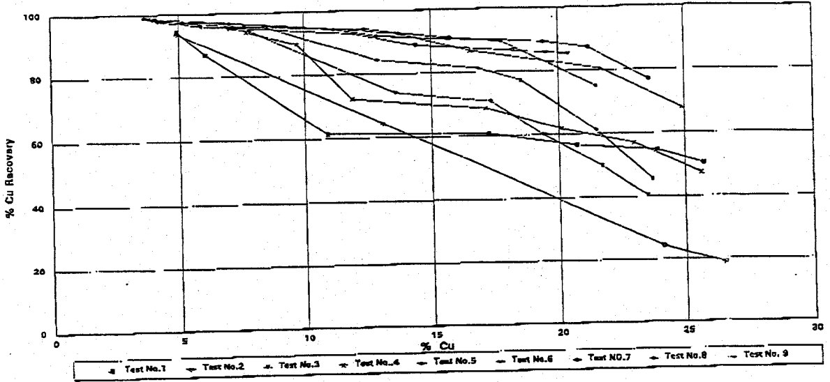
FIGURE A-1 EYRE LAKE PROJECT FLOTATION TESTS NO. 1, 2, 3, 4, 5, 6, 7, 8 AND 9 COPPER RECOVERY vs % Cu in CONCENTRATE
