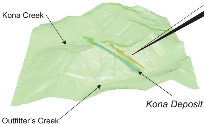
10A: Solid 3D geological model of Kona deposit with transparent topographic surface looking northward.
