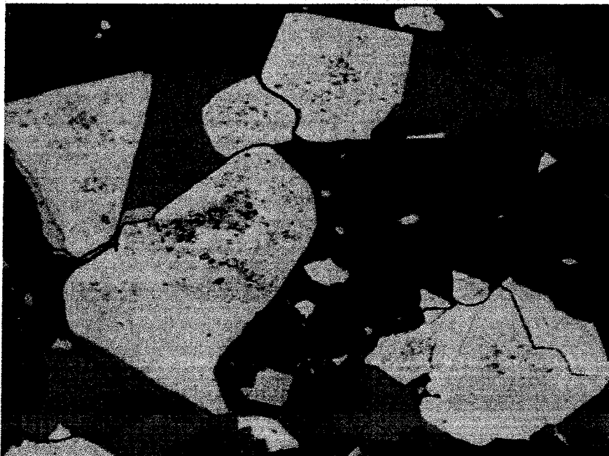
Photo 2. Fyre Lake Deposit PS6506 Mag 200X Reflected Light
