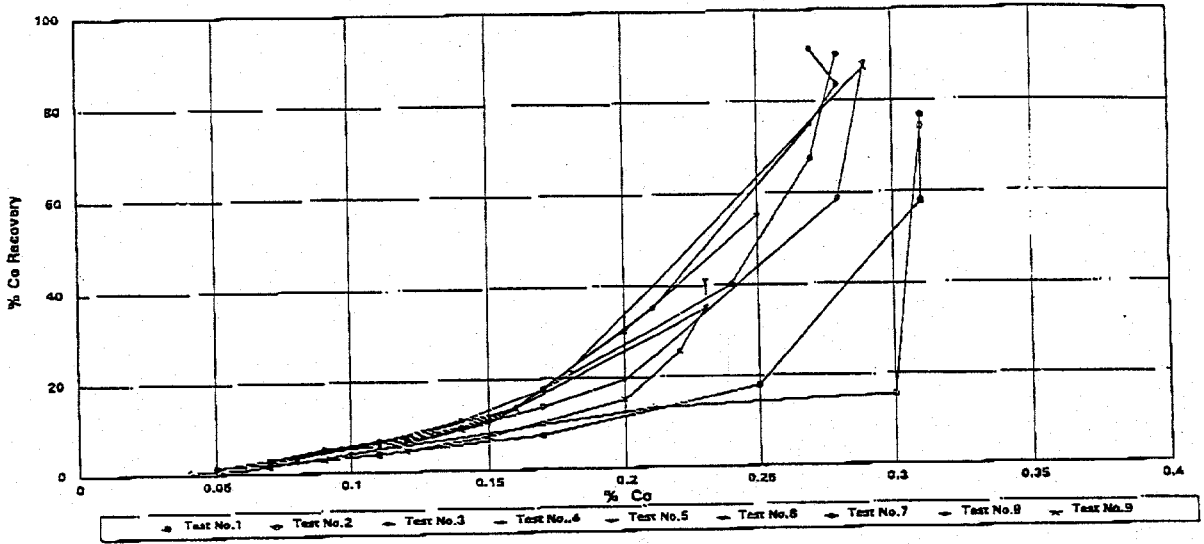
FIGURE A-4 EYRE LAKE PROJECT FLotation TESTS NO. 1, 2, 3, 4, 5, 6, 7, 8 AND 9 COBALT RECOVERY vs. % Co IN CONCENTRATE
