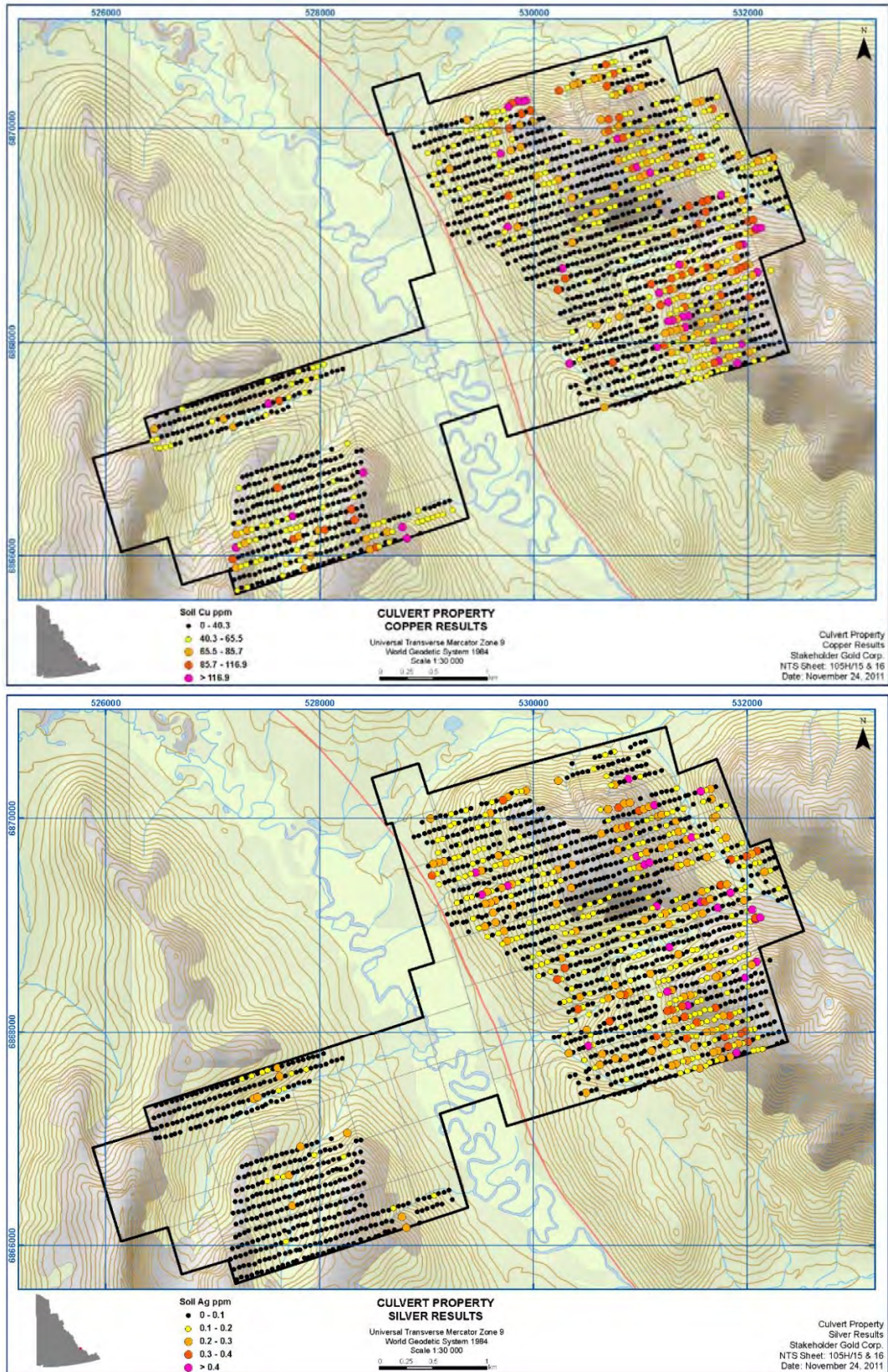
Figure 17: Copper and silver soil geochemistry results of 2011 Stakeholder program. (Fekete and Huber, 2011)
