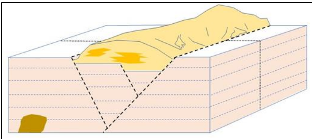
Figure 7-14: Normal and transfer faulting coeval with emplacement of felsic pile
