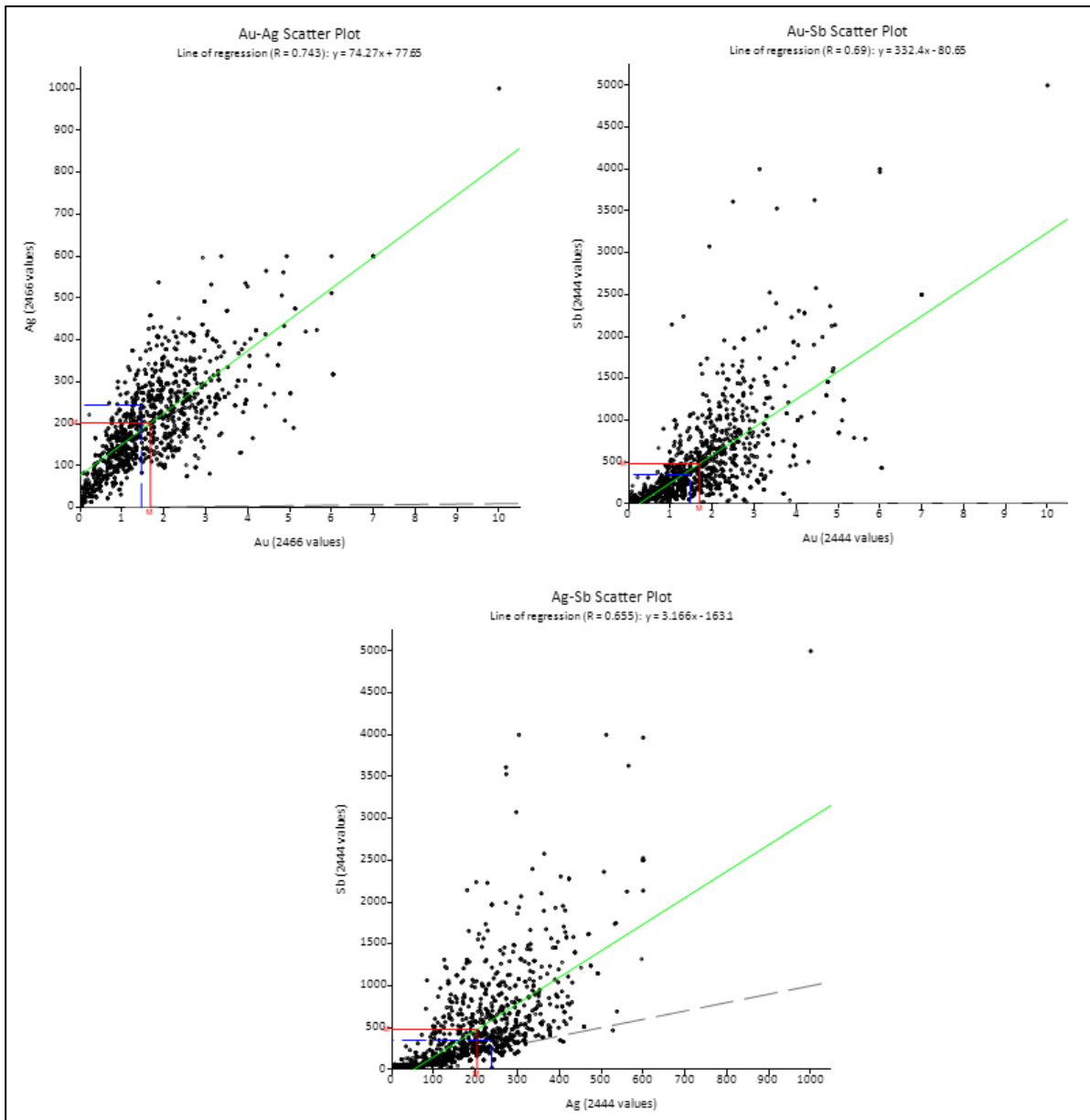
Figure 14-9: Krakatoa Zone – scattergram correlation plots for cut variables
