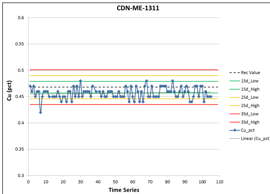
Figure 11-6: 2015 CRM (CDN-ME-1311) control chart for Cu (%) showing negative bias 1Sd = 1 standard deviation, 2Sd = 2 standard deviations, 3Sd = 3 standard deviations as defined for the individual CRM.
