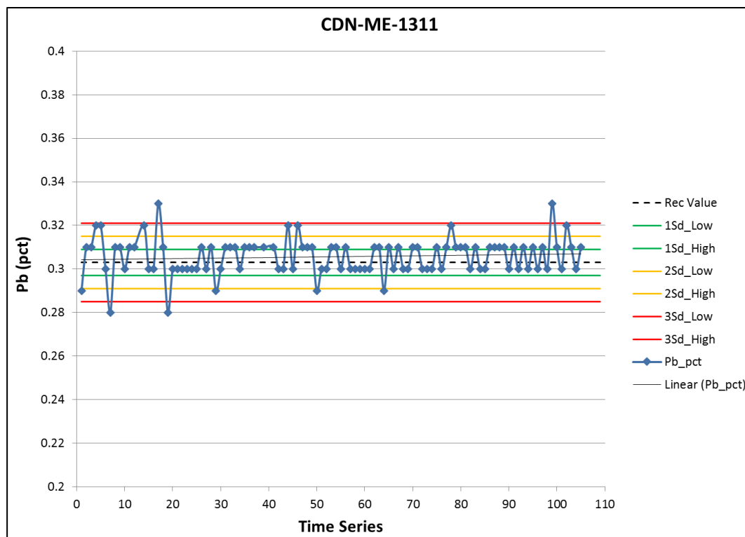
Figure 11-7: 2015 CRM (CDN-ME-1311) control chart for Pb (%) showing slight positive bias 1Sd = 1 standard deviation, 2Sd = 2 standard deviations, 3Sd = 3 standard deviations as defined for the individual CRM.
