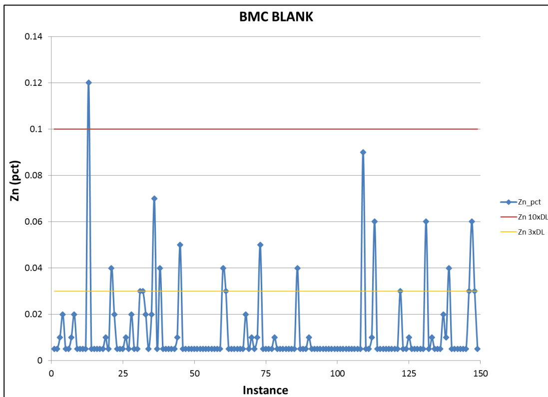
Figure 11-5: Blank control chart for Zn (%)
