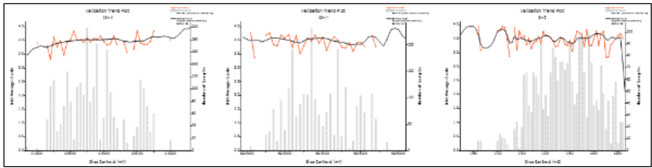
Figure 14-14: Swath plot by 30 m easting, 10 m northing, and 5 m bench, for the Krakatoa Zone bulk density
