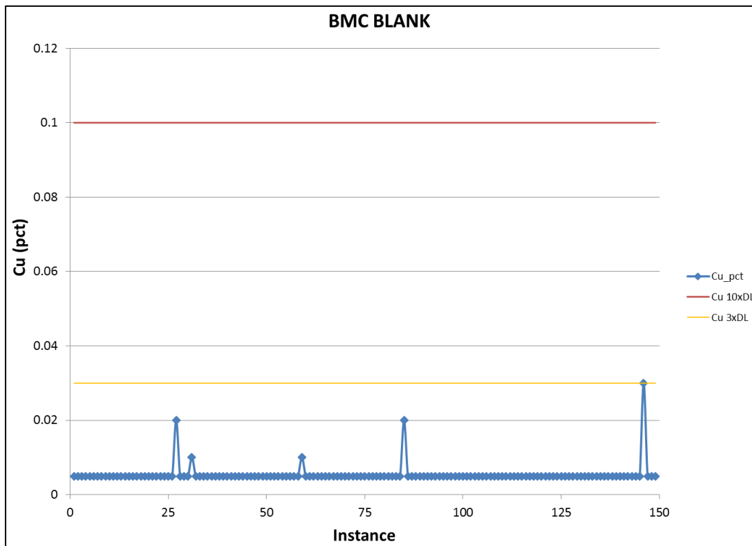
Figure 11-4: Blank control chart for Cu (%)
