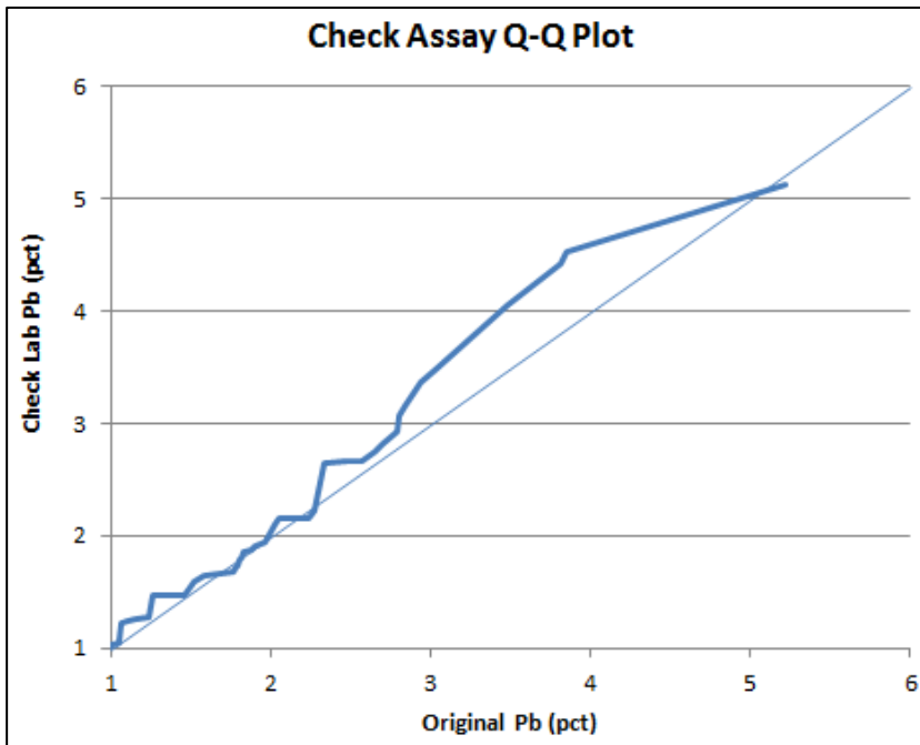
Figure 11-12: Quantile-quantile (Q-Q) plot using each data pair as a quantile and showing different distributions for Pb data from ALS and SGS
