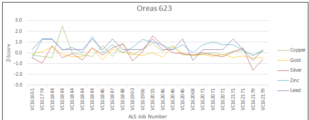
Figure 11-10: 2016 ABM Zone summary of Z-score for OREAS 623
