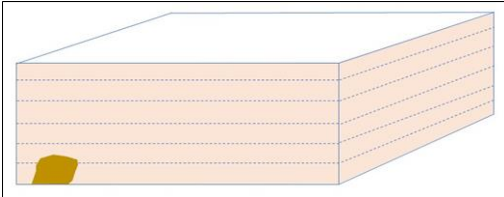
Figure 7-13: Deposition of stratified volcanoclastics as mass flows distal to a felsic volcanic source
