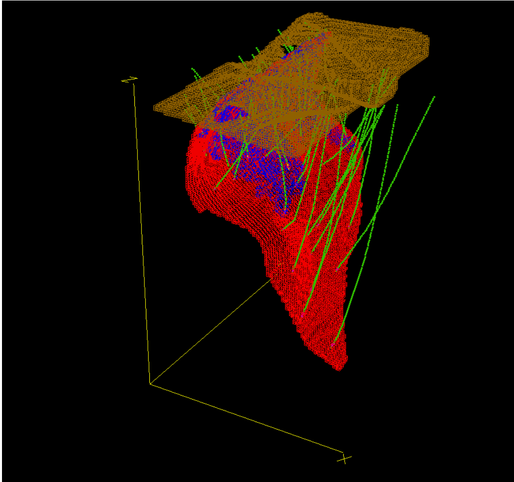
Figure 14.5: View looking NW showing block model with overburden in brown, Mineralized Solid in red, Barite Shell in blue and drill hole traces.
