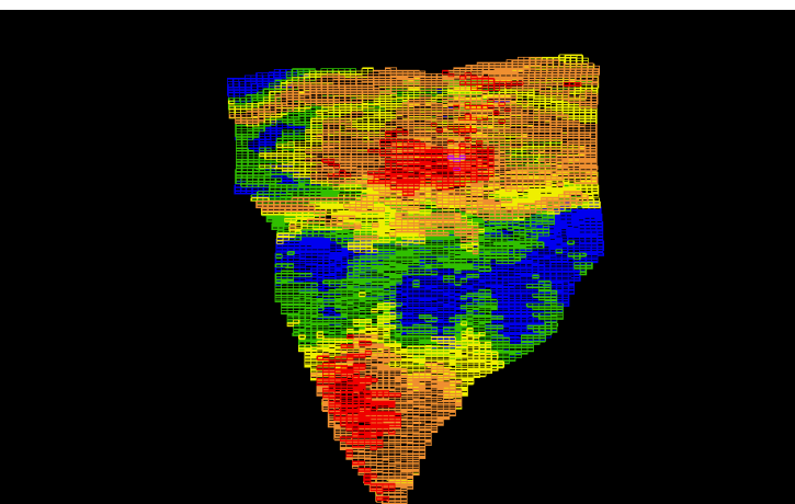
Figure 14.7: Long sections showing estimated Zn, Pb and Ba blocks colour coded by grade
