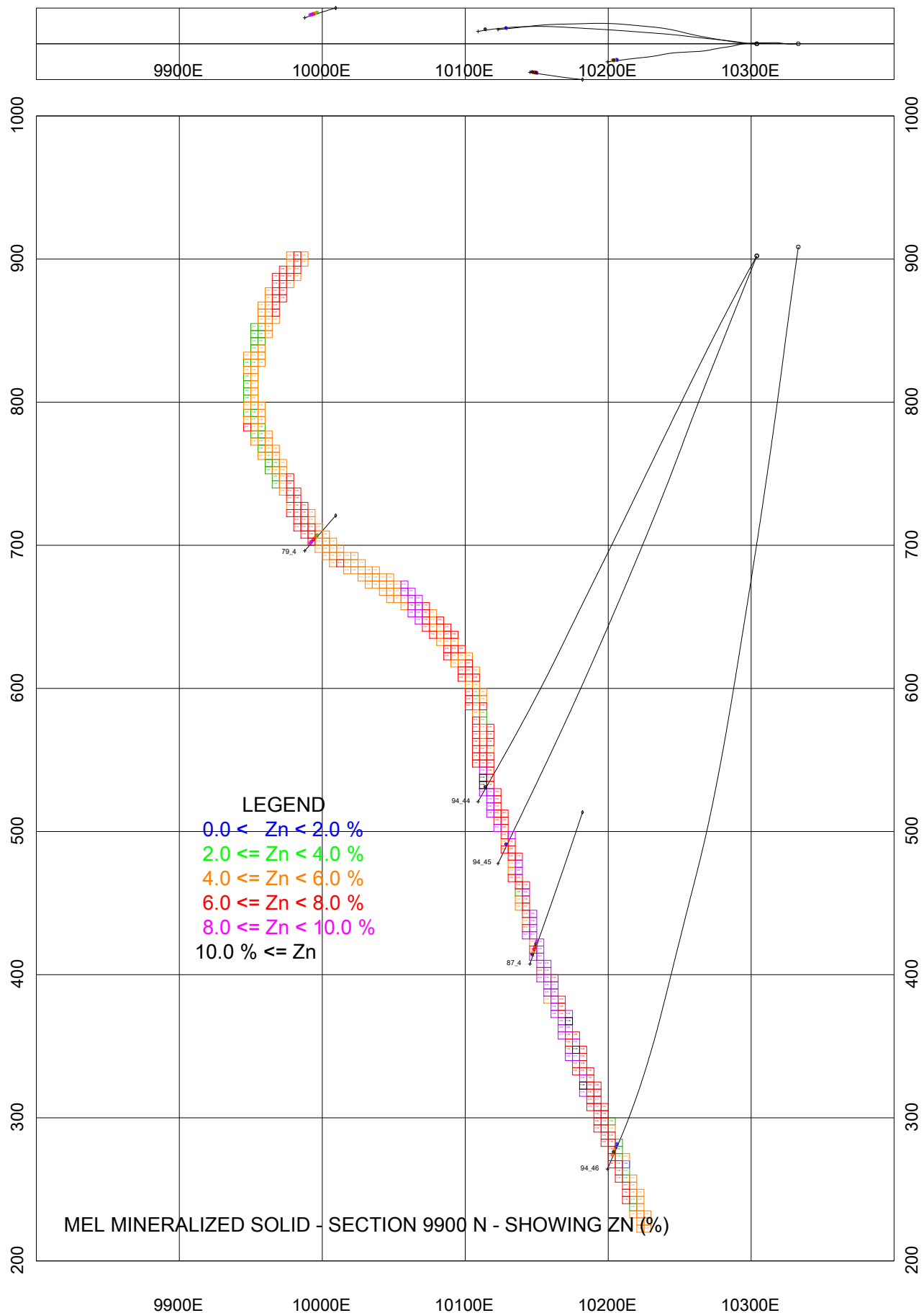
Figure 14.10: Section 9900 N showing composites and estimated Zn blocks
