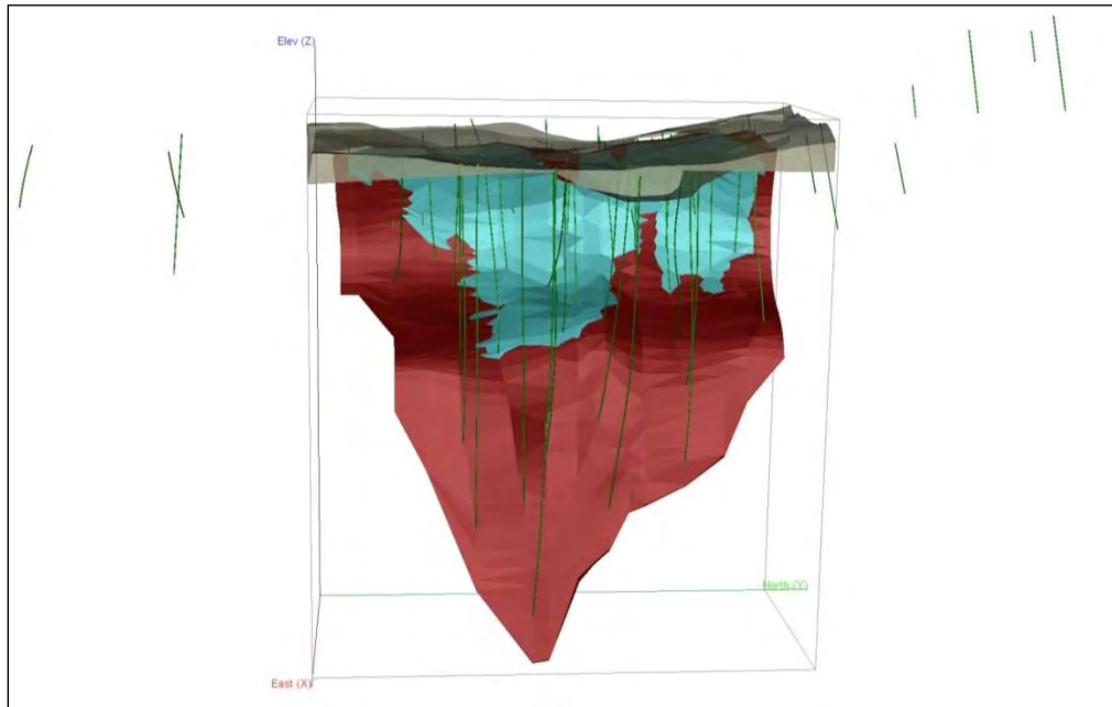
Figure 14.1: Isometric view looking W showing Mineralized Solid in red, Barite Shell in blue, surface topography, overburden surface and drill hole traces.
