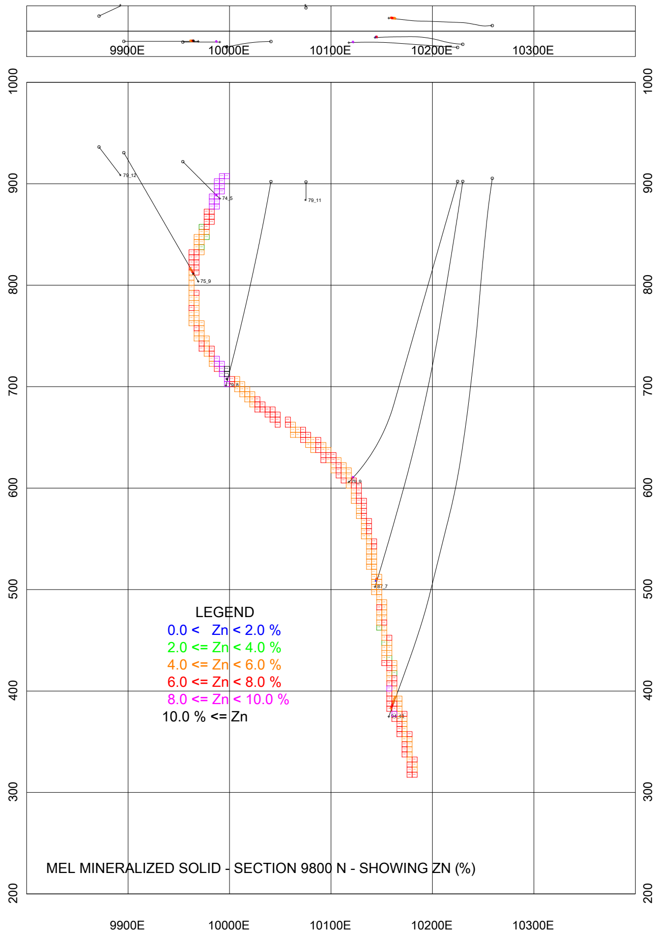
Figure 14.11: Section 9800 N showing composites and estimated Zn blocks
