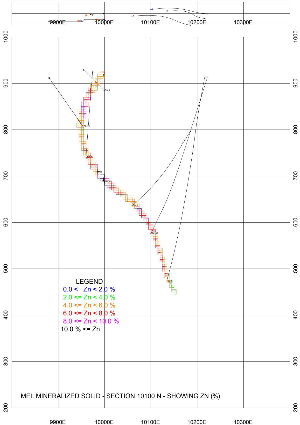
Figure 14.8: Section 10100 N showing composites and estimated Zn blocks
