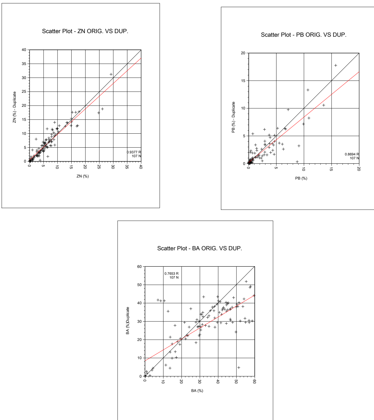
Figure 14.3: Scatter plots for Original assays versus Duplicates
