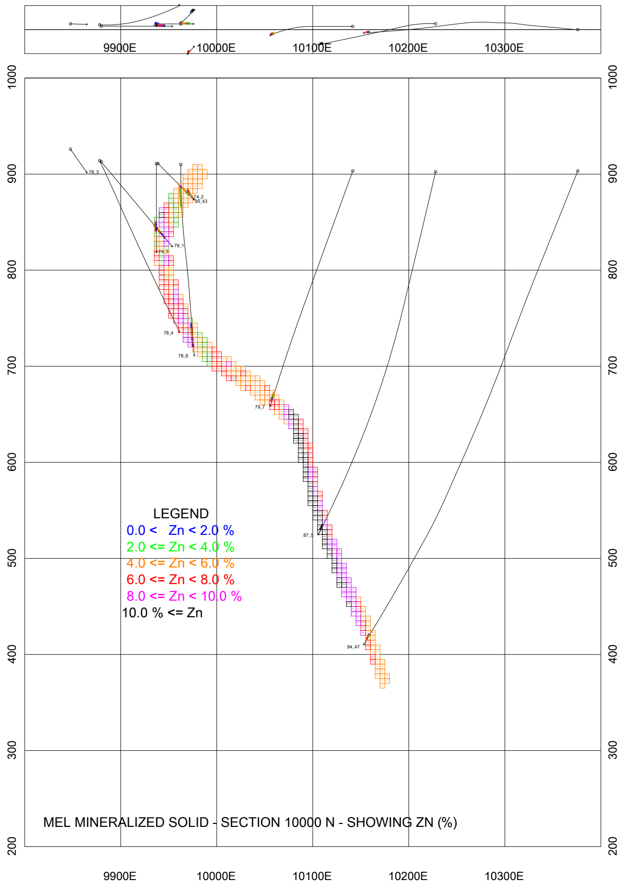
Figure 14.9: Section 10000 N showing composites and estimated Zn blocks
