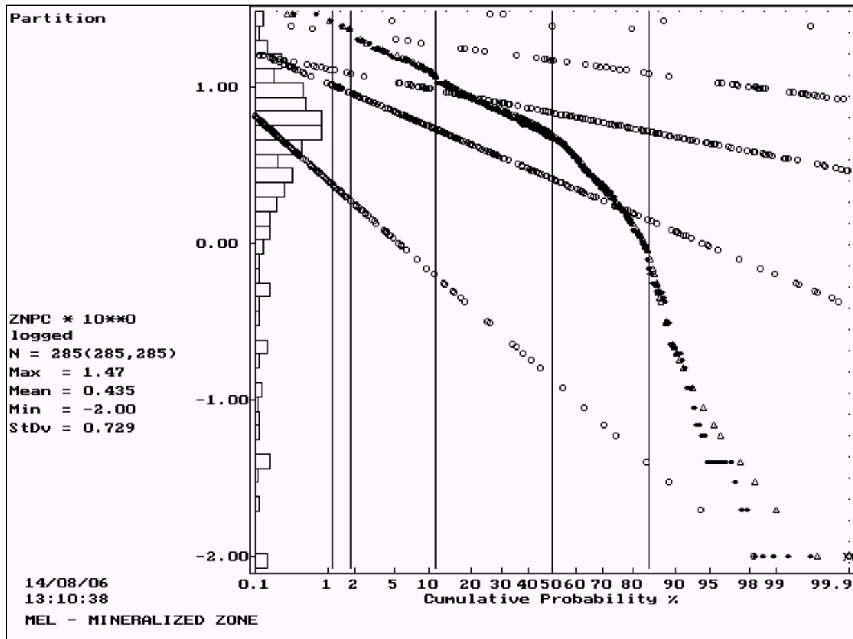
Figure 14.4: Lognormal cumulative frequency plot for Zn in Mineralized Solid
