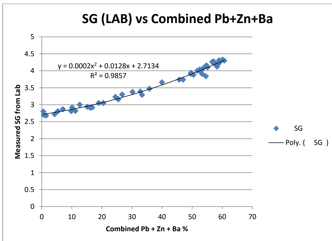
Figure 14.6: Scatter plot of Lab SG vs Combined Pb + Zn + Ba %
