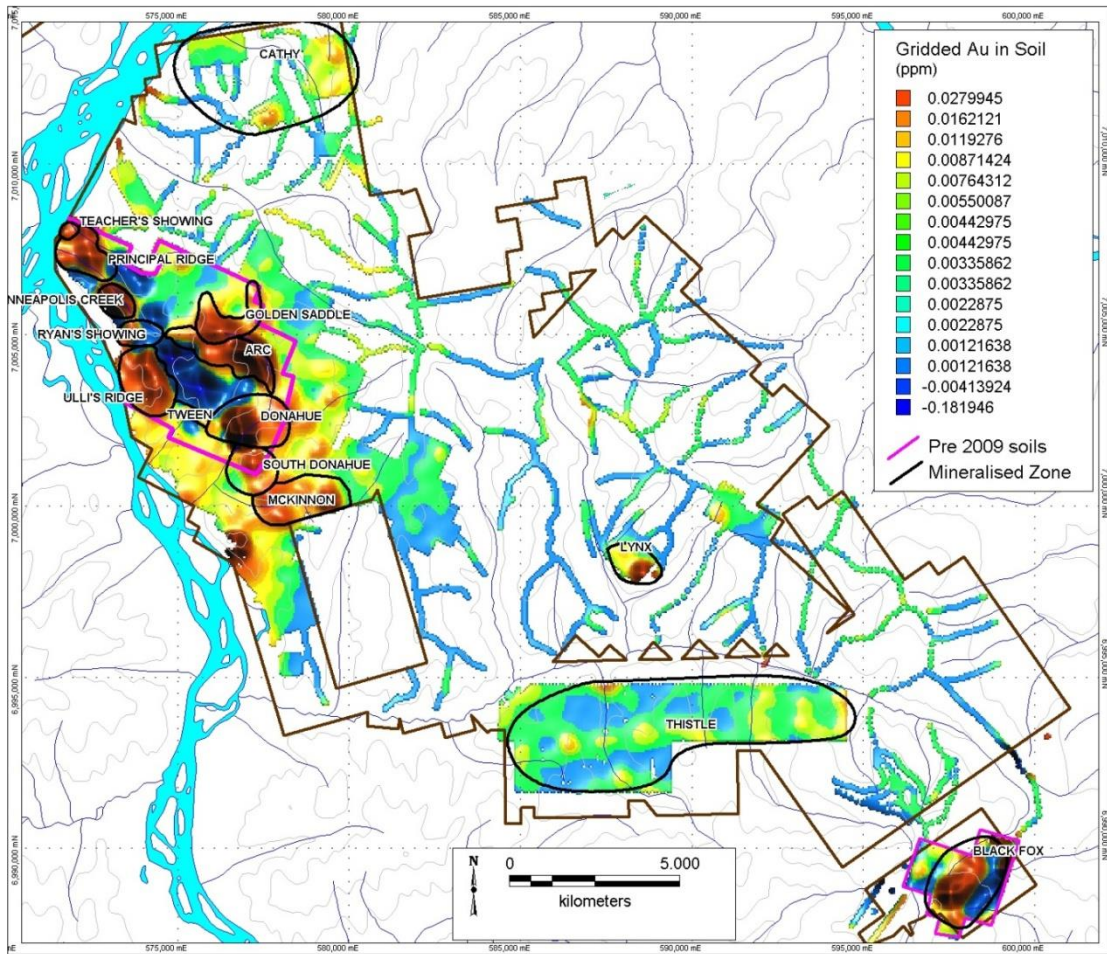
Source: SRK (2010) Figure 6.6 Geochemistry of the main White block with gridded Au soil geochemistry
