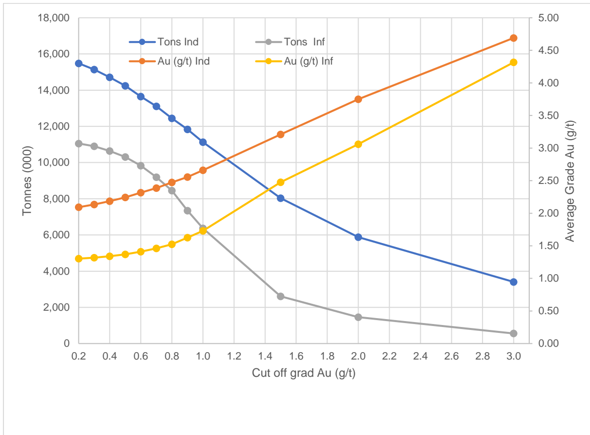
Figure 14.11 Grade Tonnage Curves for Golden Saddle and Arc deposits
