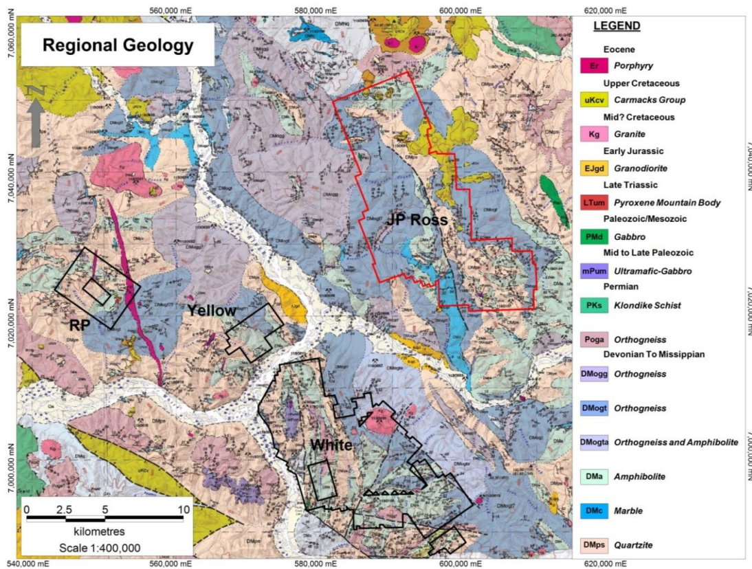
Figure 7.2 Regional geology of White Gold Project
