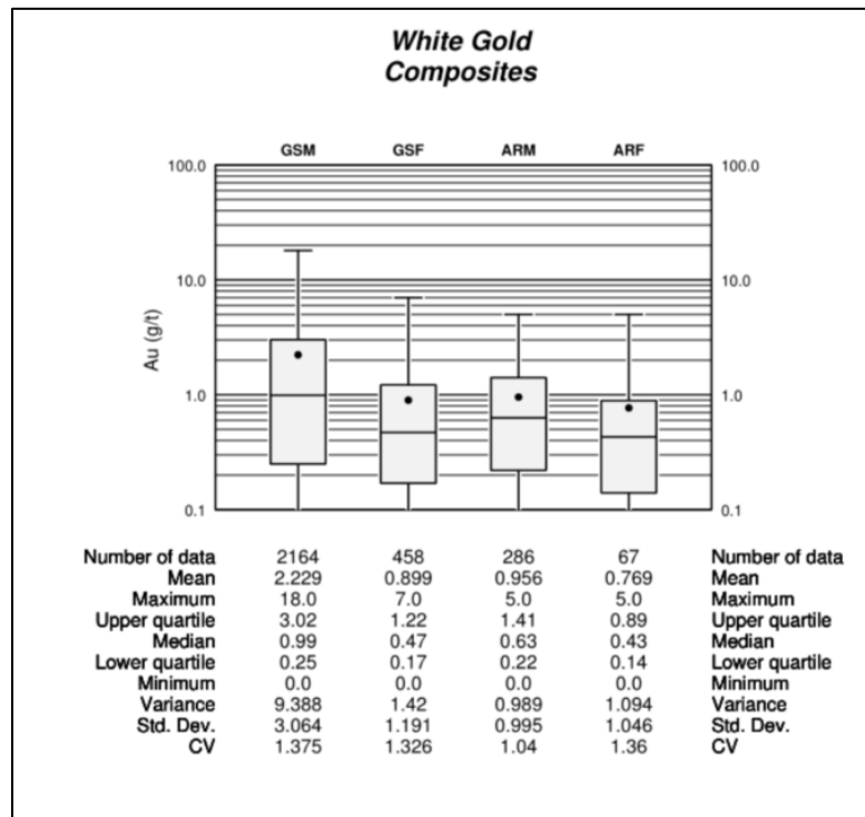
Figure 14.4 Basic statistics for capped gold composited assay data for Golden Saddle Main (GSM), Golden Saddle Footwall (GSF), Arc Main (ARM) and Arc Footwall (ARF)
