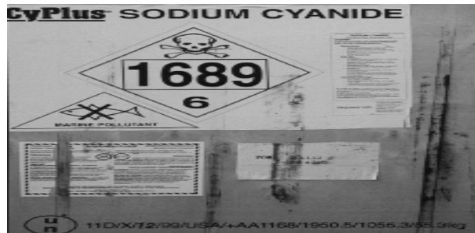
A container of sodium cyanide in solid "briquette" form.
