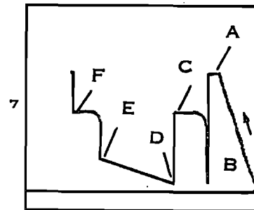
7 The chart shows the equalizing, the by-pass ports have been opened permitting the drilling fluid to flow through the packer to the test zone. Thus, pressure is equalized above and below the packer. The equalization of the pressure facilitates easier removal of the packer from the packer seat.
