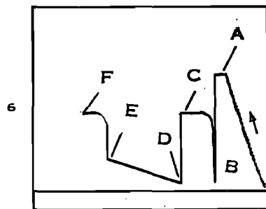
6 The final shut-in pressure is taken by stopping the flow of formation fluid into the drill pipe. Note the characteristic build-up curve. The well bore pressure is approaching equilibrium with the static reservoir pressure. When the shut-in curve levels-off the static reservoir pressure has been reached.
