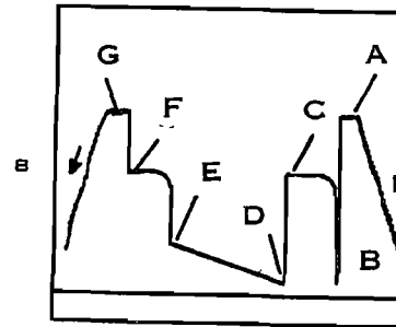
8 The packer has been unseated. The testing assembly is being removed from the hole.
