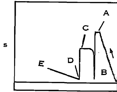
5 The pressure of fluid flowing from the formation into the well bore, through the perforated anchor, and into the drill pipe, is recorded on the chart.
