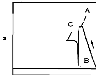
3 This chart shows the initial shut-in pressure. There is one mechanical method commonly used to obtain this pressure. A 4 stage shut-in tool, that is run-in in the open position and rotated closed when the desired amount of initial flow time is obtained. This initial shut-in pressure is the best method yet devised for recording the original undisturbed reservoir pressure of a formation.
