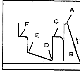
7 The chart shows the equalizing, the by-pass ports have been opened permitting the drilling fluid to flow through the packer to the test zone. Thus, pressure is equalized above and below the packer. The equalization of the pressure facilitates easier removal of the packer from the packer seat.
