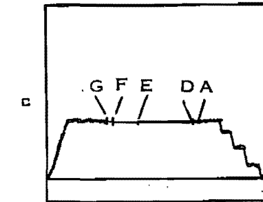
C In this case a recorder has been run above the main tester valve with a fluid cushion used in the drill pipe. No pressure is recorded as the testing tool is being lowered into the hole. Then the fluid cushion pressure is recorded as the drill pipe is filled with fluid. As more stands are run into the hole, the recorder registers the hydrostatic pressures of the cushion. When the main testing valve is opened the pressure of the cushion column or the flowing pressure of the formation, (which ever is greater), is recorded.
