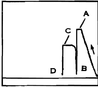
4 The chart indicates a pressure drop. The test tool has been opened to the surface by rotating the 4 stage shut-in tool into the open position. Permitting the open formation to produce.
