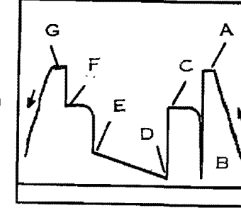
8 The packer has been unseated. The testing assembly is being removed from the hole.
