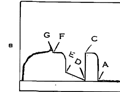
B In this case a recorder has been run in an air chamber. The hydrostatic mud pressures are not influencing the recorder while going in or coming out of the hole due to the main tester valve being closed. The flow pressures and shut-in pressures are recorded while the main tester valve is opened.
