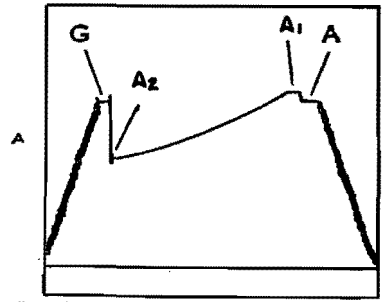
A The above is a typical illustration of a chart from a recorder that is run below the bottom packer on a conventional straddle test. Only the hydrostatic mud pressures are recorded. When the tool is opened, there is a pressure differential across the bottom packer. This differential is lessened by the rubber flow of the packer element, which in turn causes a draw-down in pressure. If the below straddle chart reads the same as a chart that is run to record pressures of the test zone, then the bottom packer has failed. If this occurs, all zones below the top packer are being tested.
