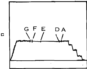
In this case a recorder has been run above the main tester valve with a fluid cushion used in the drill pipe. No pressure is recorded as the testing tool is being lowered into the hole. Then the fluid cushion pressure is recorded as the drill pipe is filled with fluid. As more stands are run into the hole, the recorder registers the hydrostatic pressures of the cushion. When the main testing valve is opened the pressure of the cushion column or the flowing pressure of the formation, (which ever is greater), is recorded.
