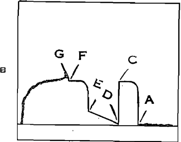
In this case a recorder has been run in an air chamber. The hydrostatic mud pressures are not influencing the recorder while going in or coming out of the hole due to the main tester valve being closed. The flow pressures and shut-in pressures are recorded while the main tester valve is opened.
