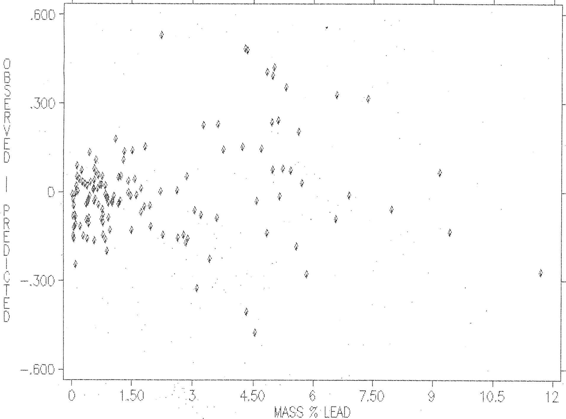
STEPWISE LINEAR REGRESSION ON SPECIFIC GRAVITY FAR09D DATA.
