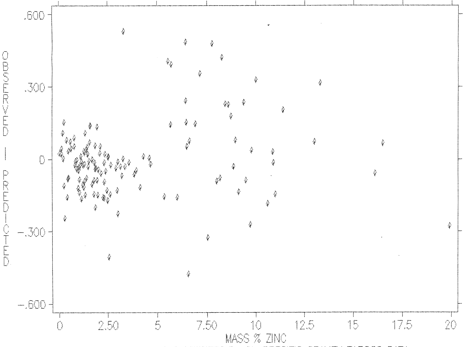
STEPWISE LINEAR REGRESSION ON SPECIFIC GRAVITY FARO90 DATA.
