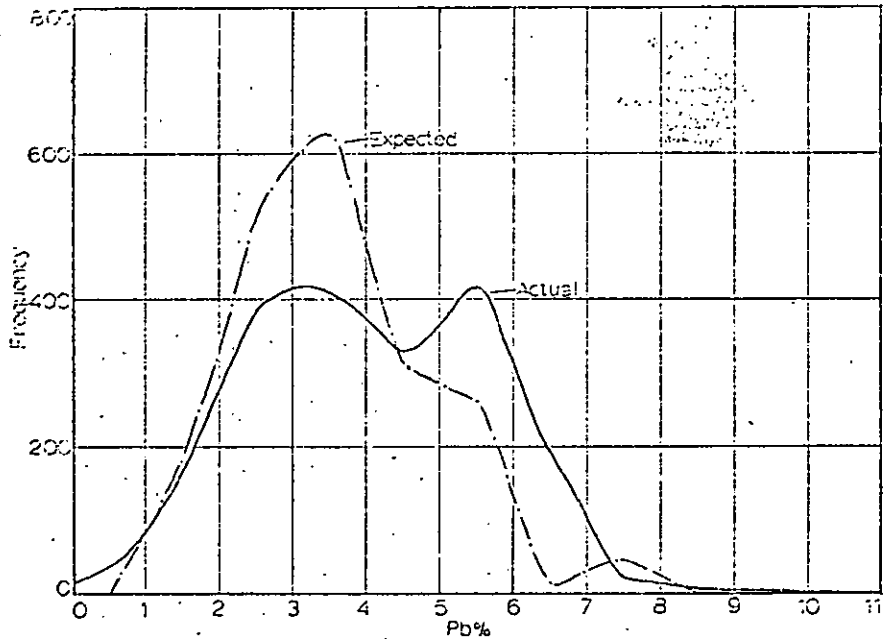
Figure 4: "Actual" (blast hole-derived) and "expected" (DDH-derived) frequency distributions showing the frequency of Pb assays reported and expected from ore mined Jan. - Dec., 1972
