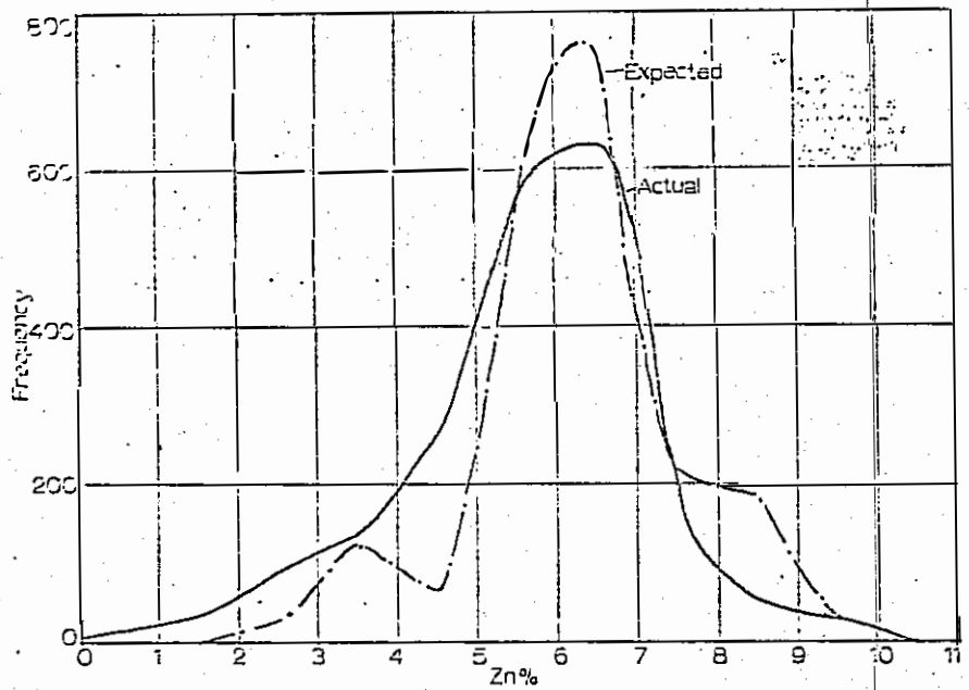
Figure 5: "Actual" (blast hole-derived) and "expected" (DDH-derived) frequency distributions showing the frequency of Zn assays reported and expected from ore mined Jan. - Dec., 1972
