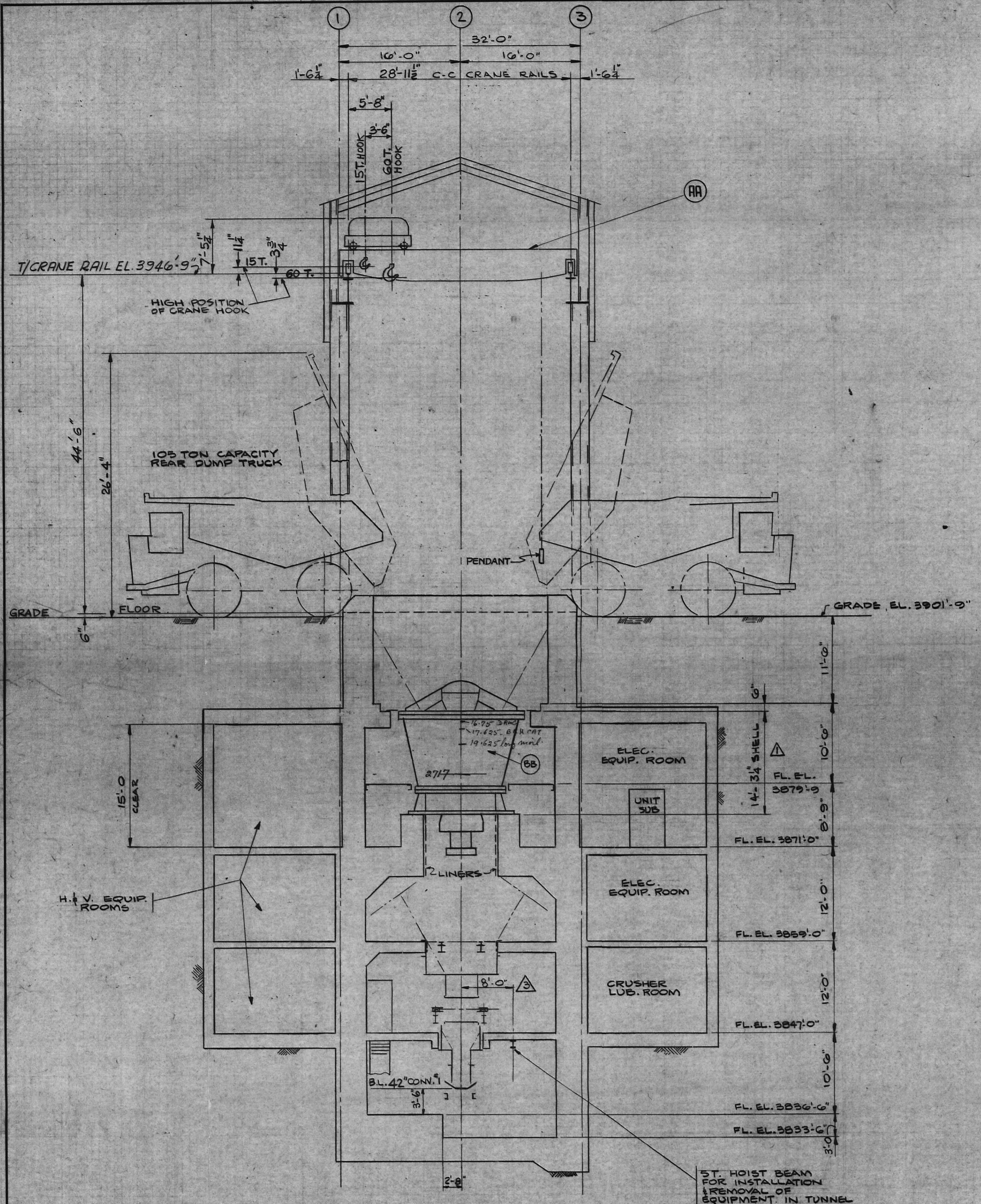
SECTION A-A LOOKING NORTH DWG. 300-1001
