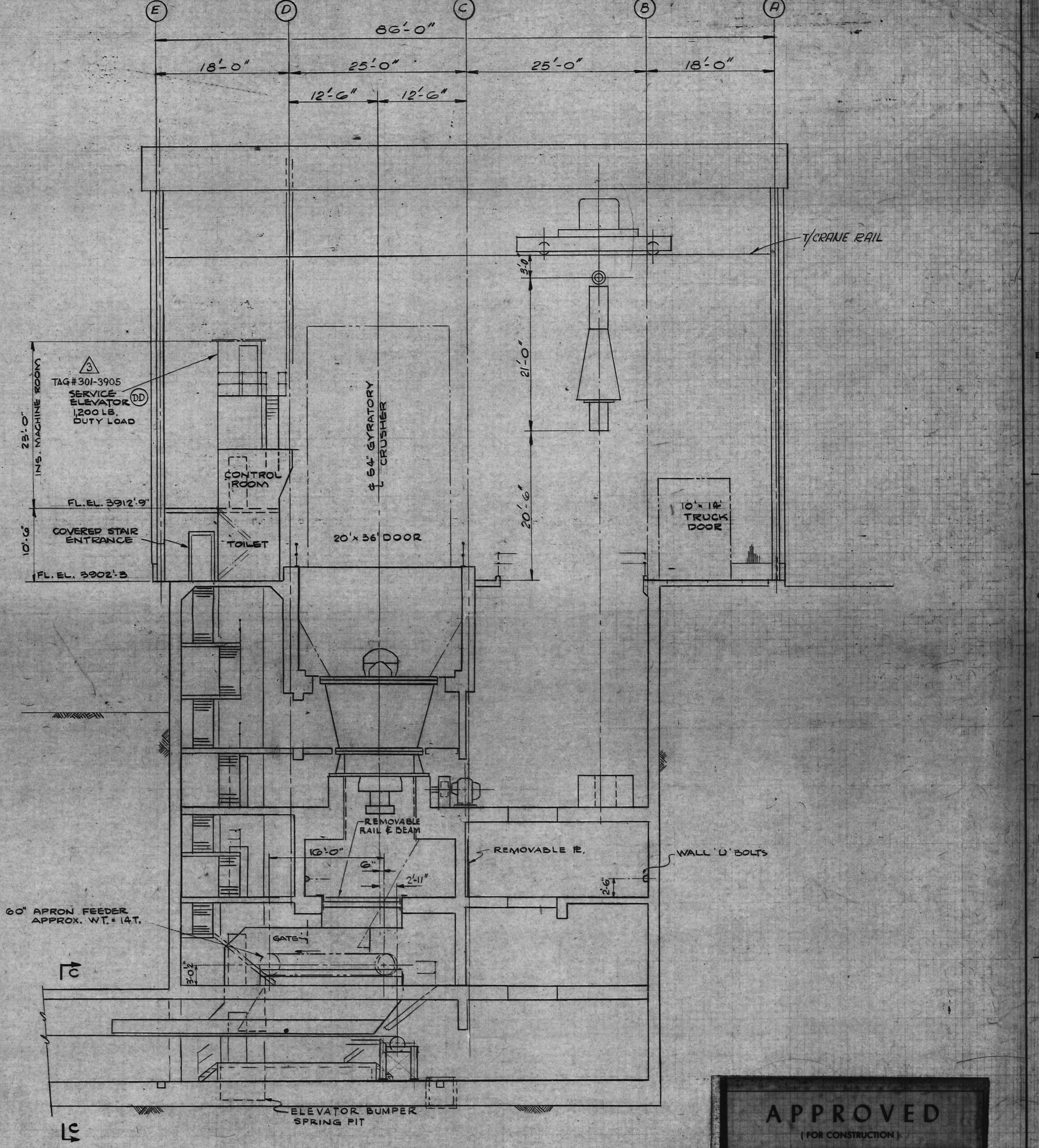
SECTION B-B LOOKING WEST DWG. 300-1001
