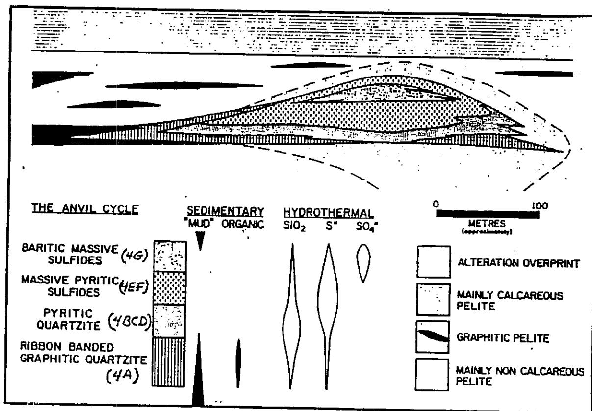
Figure 3.6 An idealized Anvil deposit based on cross sections of the Faro deposit. Such lateral and vertical zoning can be found in all deposits of the district. Massive sulphides are the central and upper lithofacies with peripheral and lower quartzose disseminated lithofacies.
