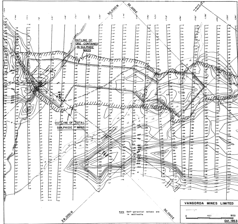
Figure 3. Self-potential survey of the lead-zinc deposit. (See page 271)
