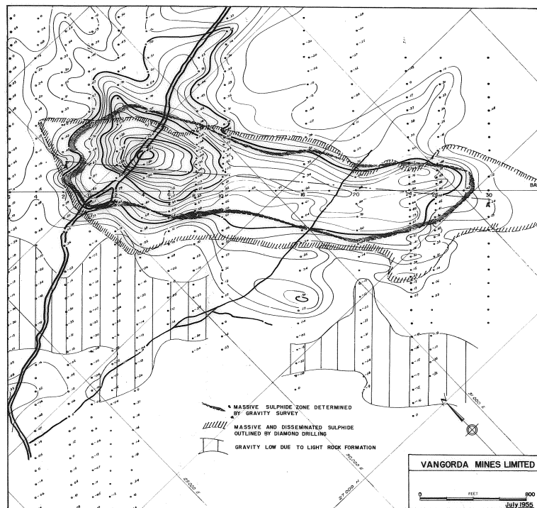
Figure 2. Map of mineral gravity over the lead-zinc deposit. (See page 271)
