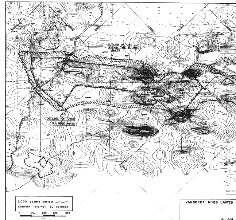
Figure 4. Magnetics survey of the lead-zinc deposit. (See page 271)
