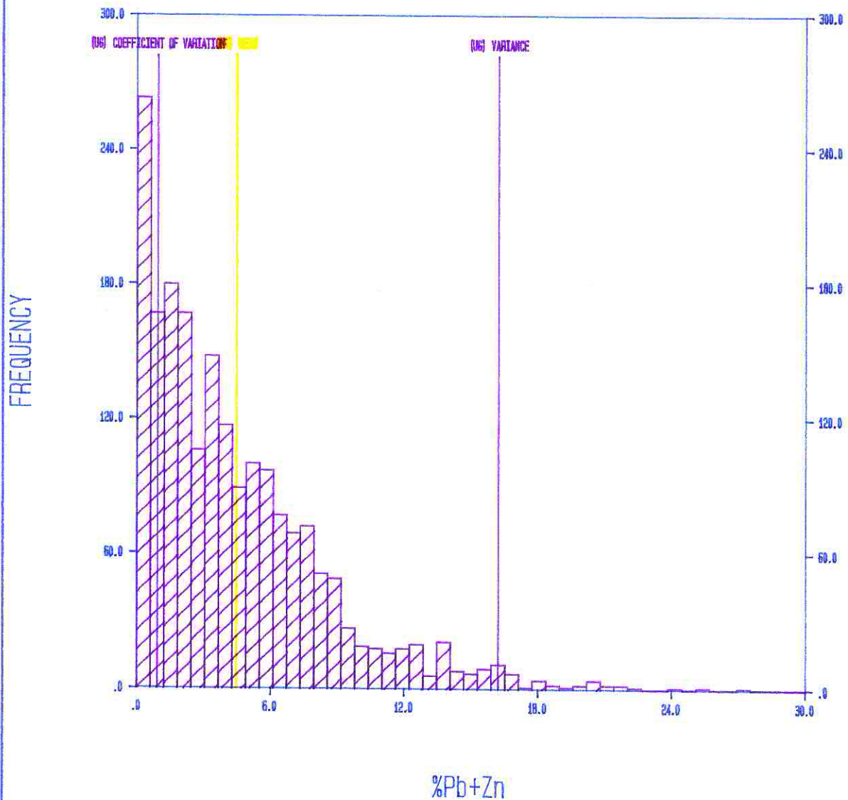
%Pb+Zn FOR ROCK CODE 20 COMPOSITES BY PARALLEL PLAINS
