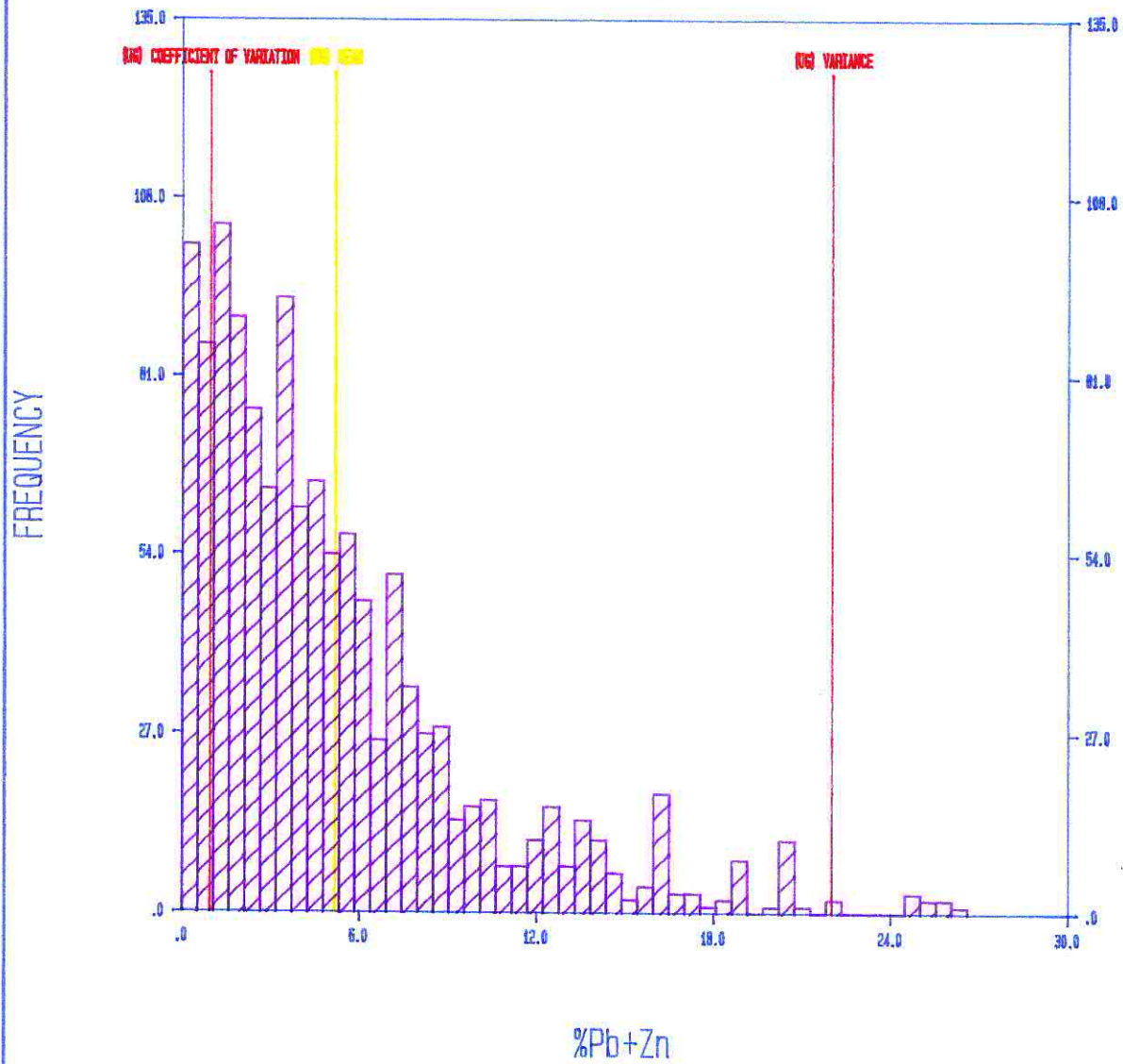
%Pb+Zn FOR ROCK CODE 30 COMPOSITES BY PARALLEL PLAINS
