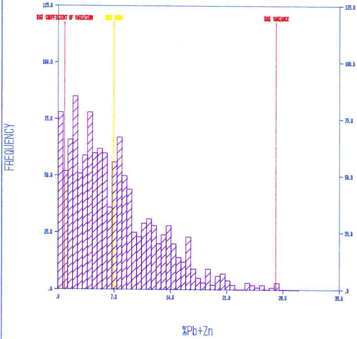
%Pb+Zn FOR ROCK CODE 50 COMPOSITES BY PARALLEL PLAINS
