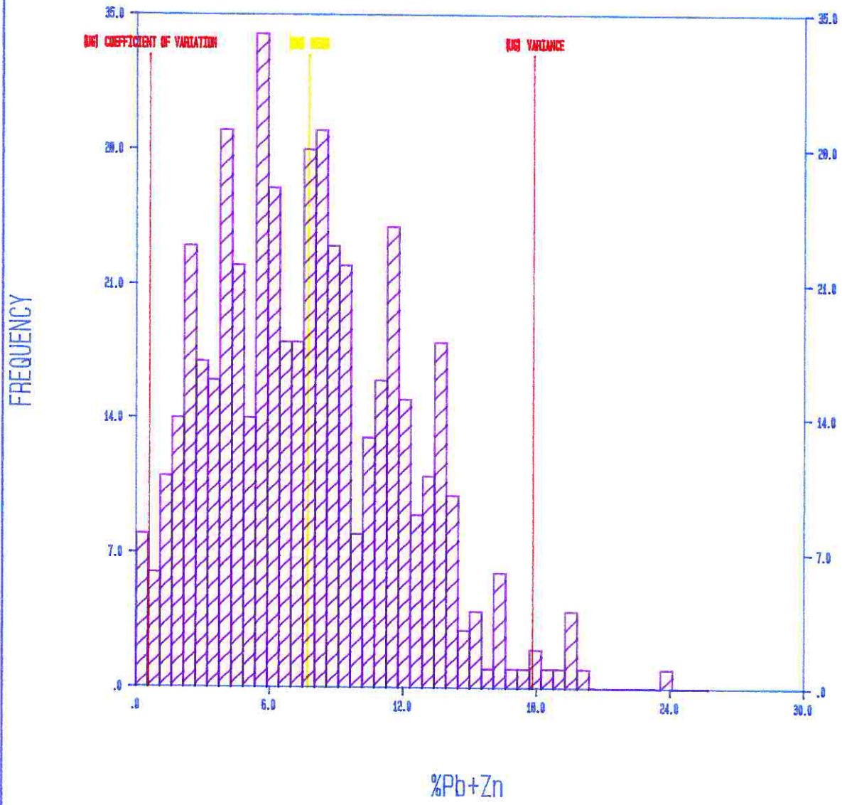
%Pb+Zn FOR ROCK CODE 60 COMPOSITES BY PARALLEL PLAINS
