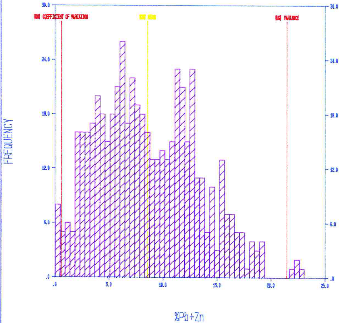
%Pb+Zn FOR ROCK CODE 60 COMPOSITES BY LENGTH
