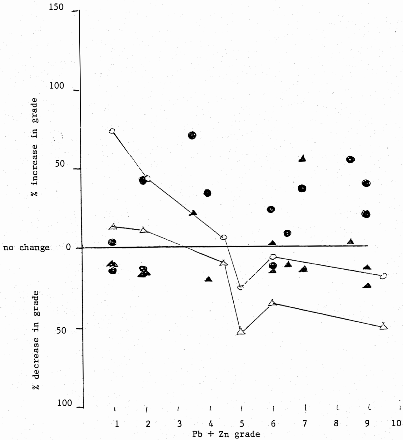
Fig. 1 Comparison of change in average lead and zinc grade between K.A. and C.A. drilling
