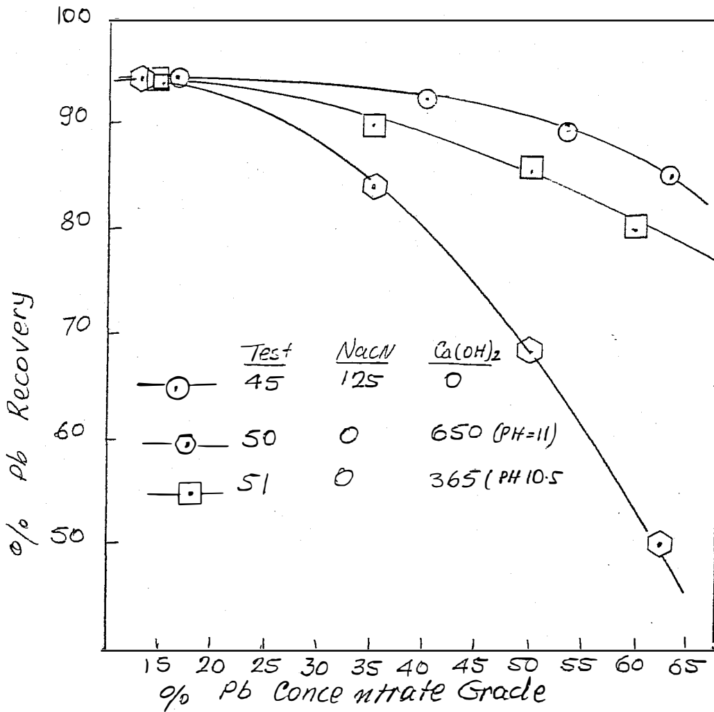
FIGURE No: Effect of Lime Additions to Pb cleaners - Comparison of Results.
