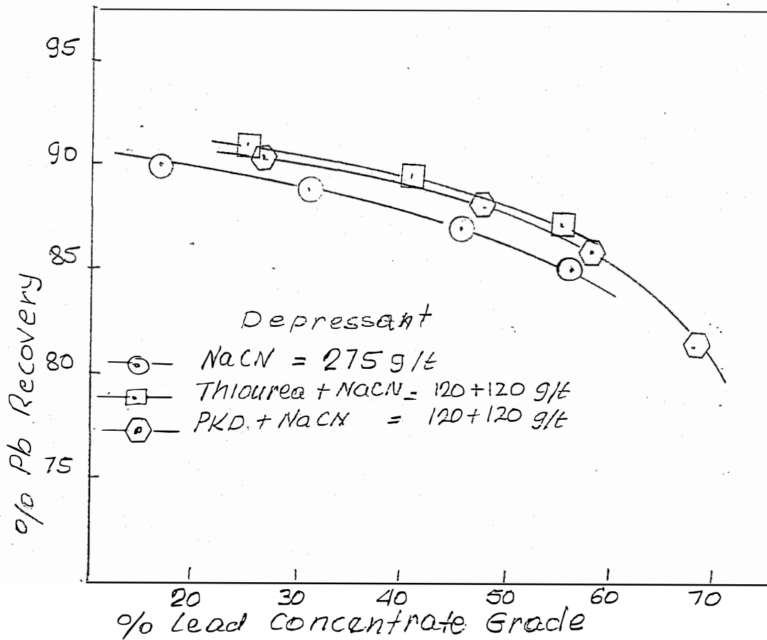
FIGURE No: EFFECT OF THIUREA AND PKD COMPLEX ON LEAD FLOTATION - G-1 ORE
