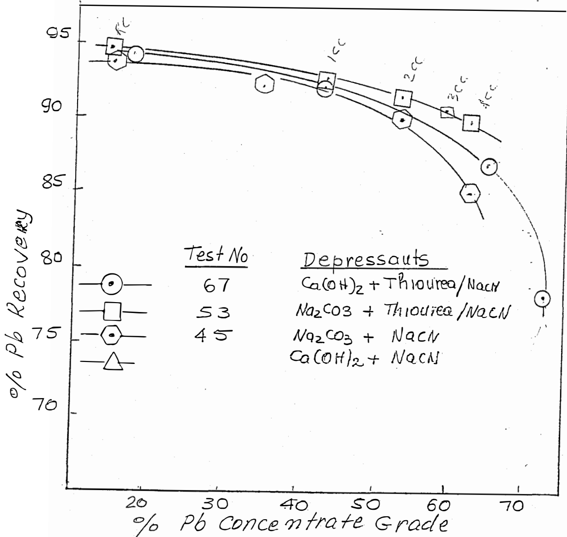
FIGURE No. 1: EFFECT OF LIME - THIUREA COMPLEX AND LIME CYANIDE ON LEAD FLOTATION - COMPARISON OF RESULTS
