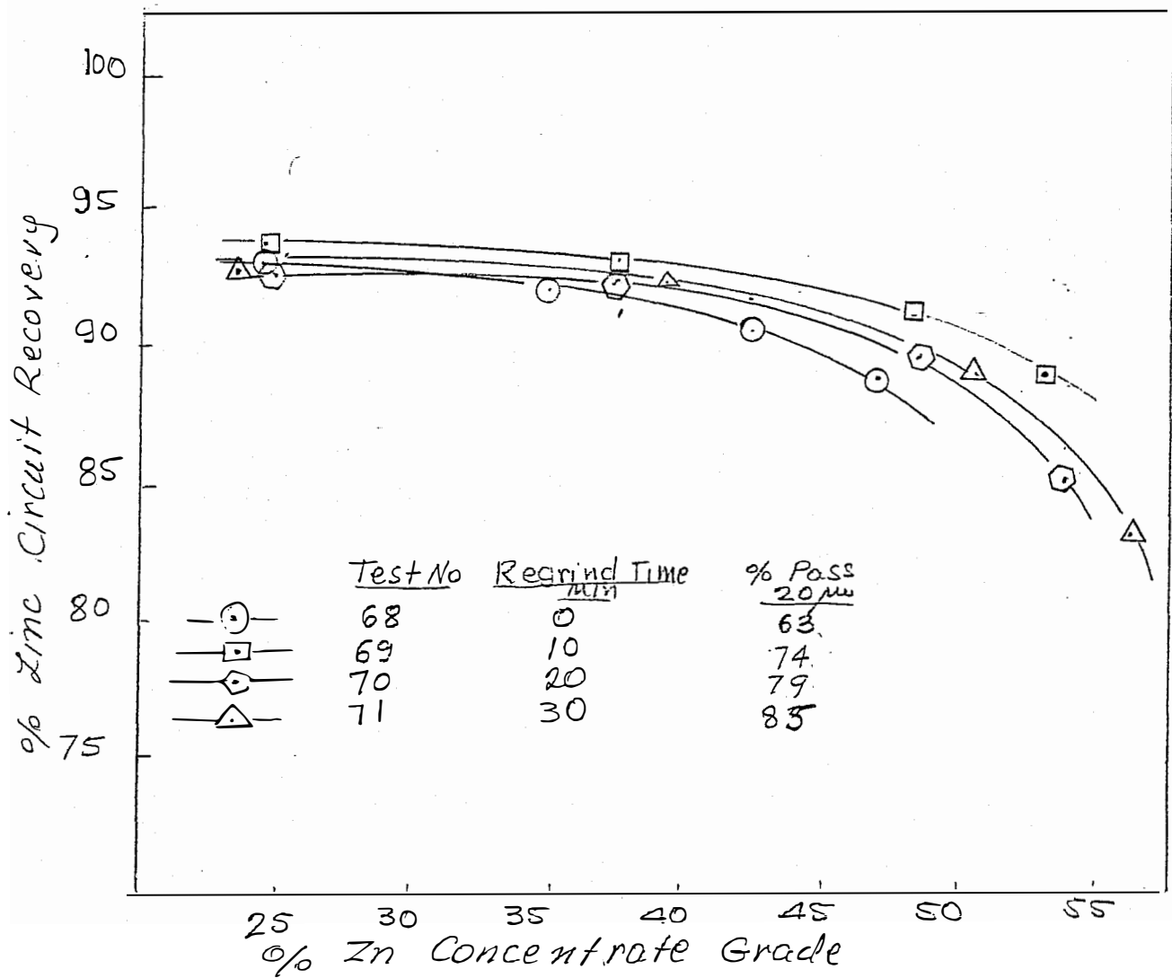
Figure No: Effect of Zinc Concentrate Regrinding on Zinc Cleaning
