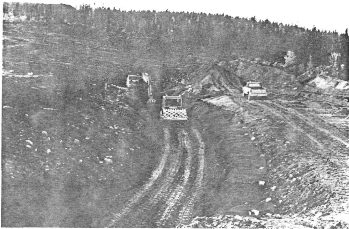
PLATE 6: Sept. 14/90. Each lift is compacted with 5 cycles of a Dynapac compactor.
