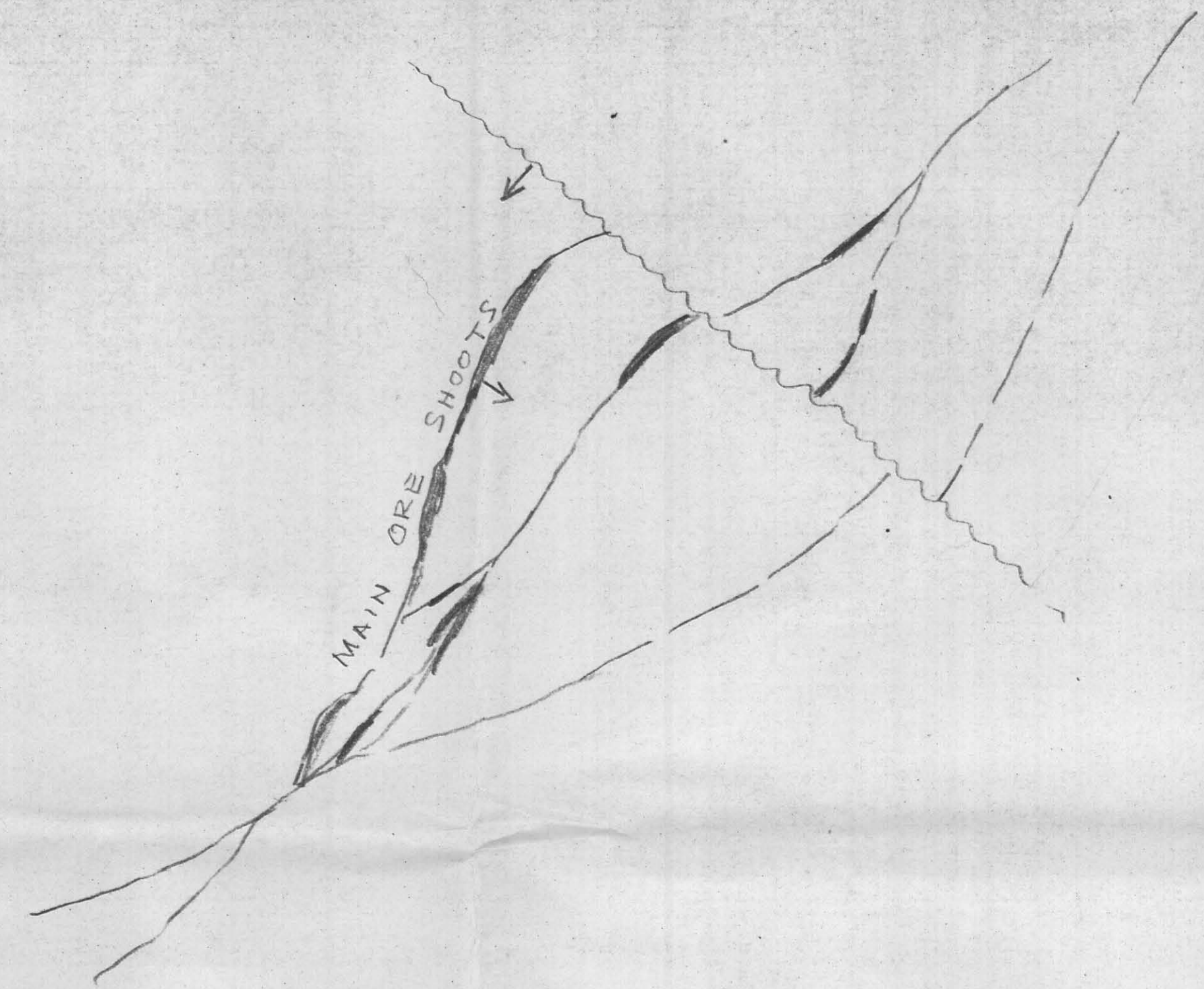
FINAL HECTOR-CALUMET TYPE ORE-BEARING VEIN-FAULT SYSTEM.
