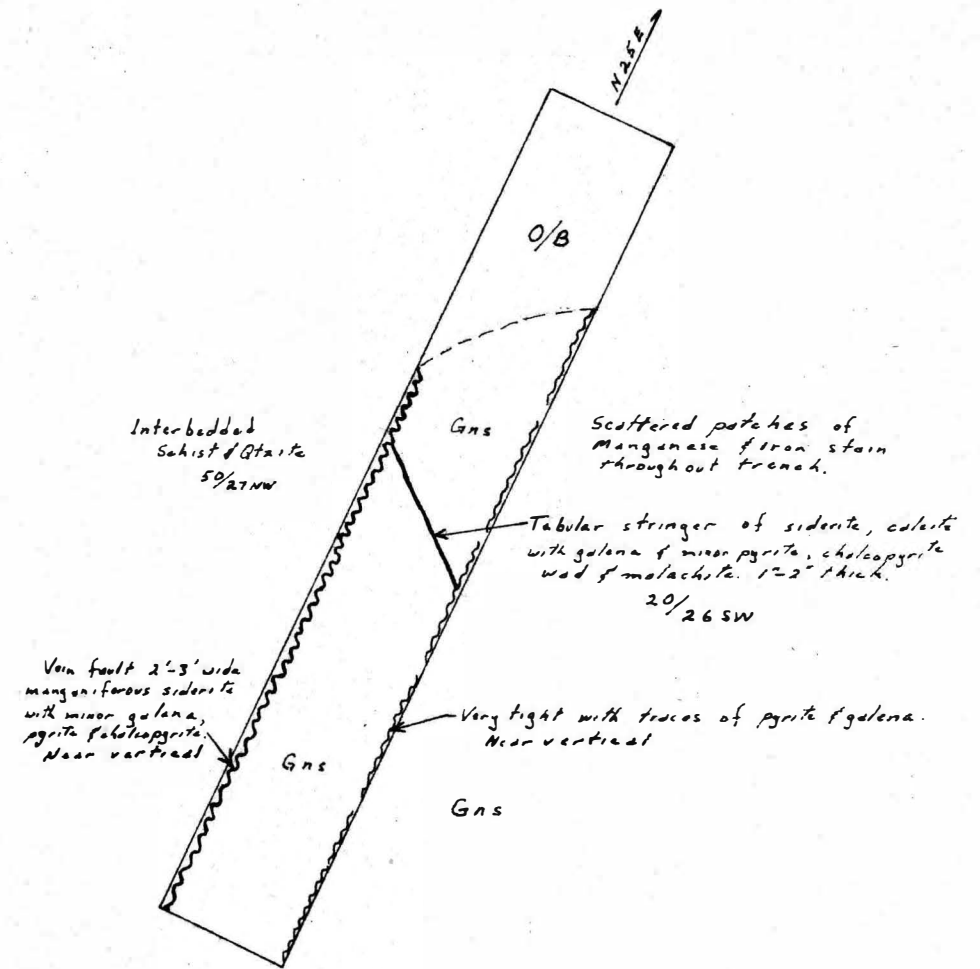
TRENCH No. 7 PLAN
