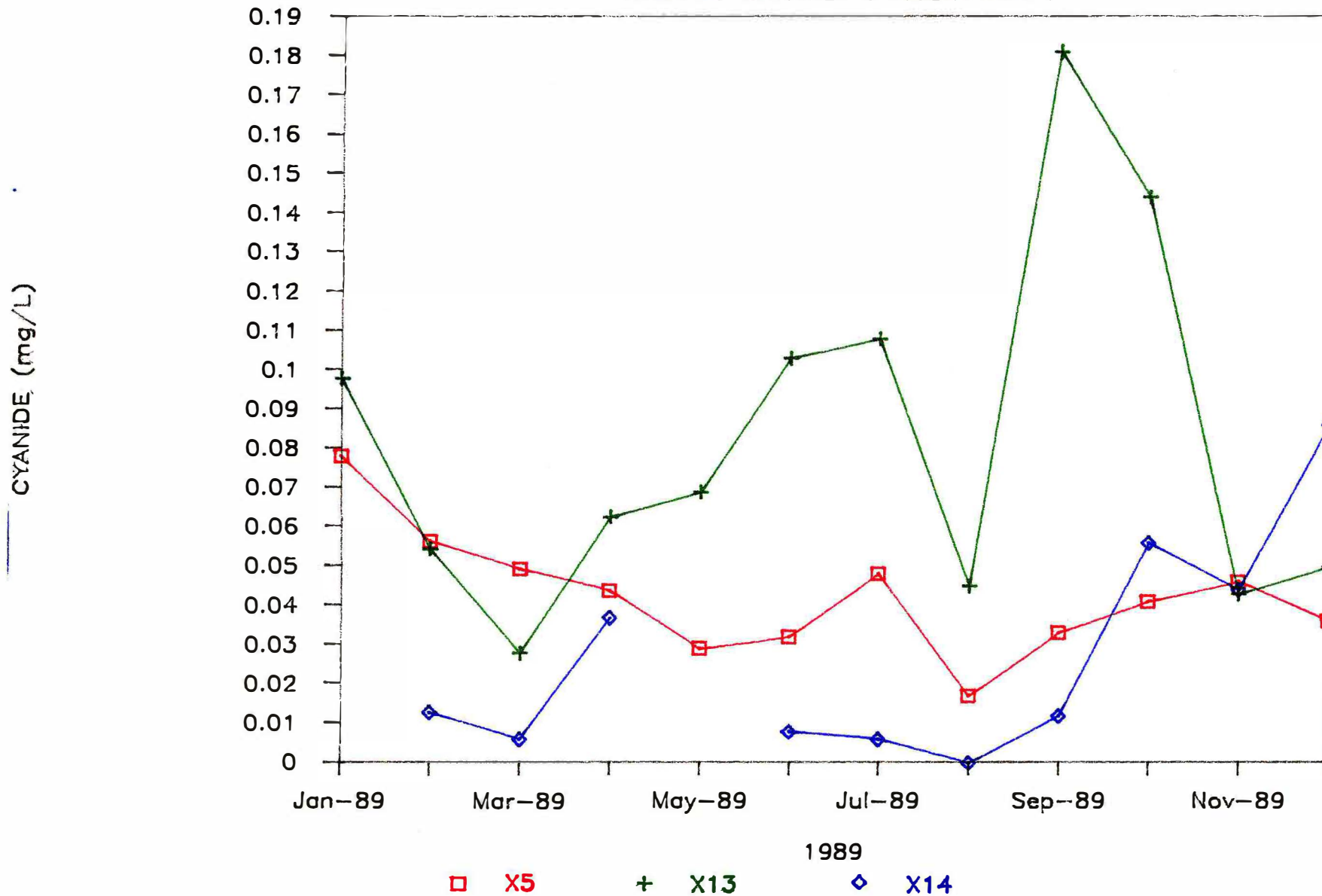
FIGURE 24 : CYANIDE (TOTAL)
