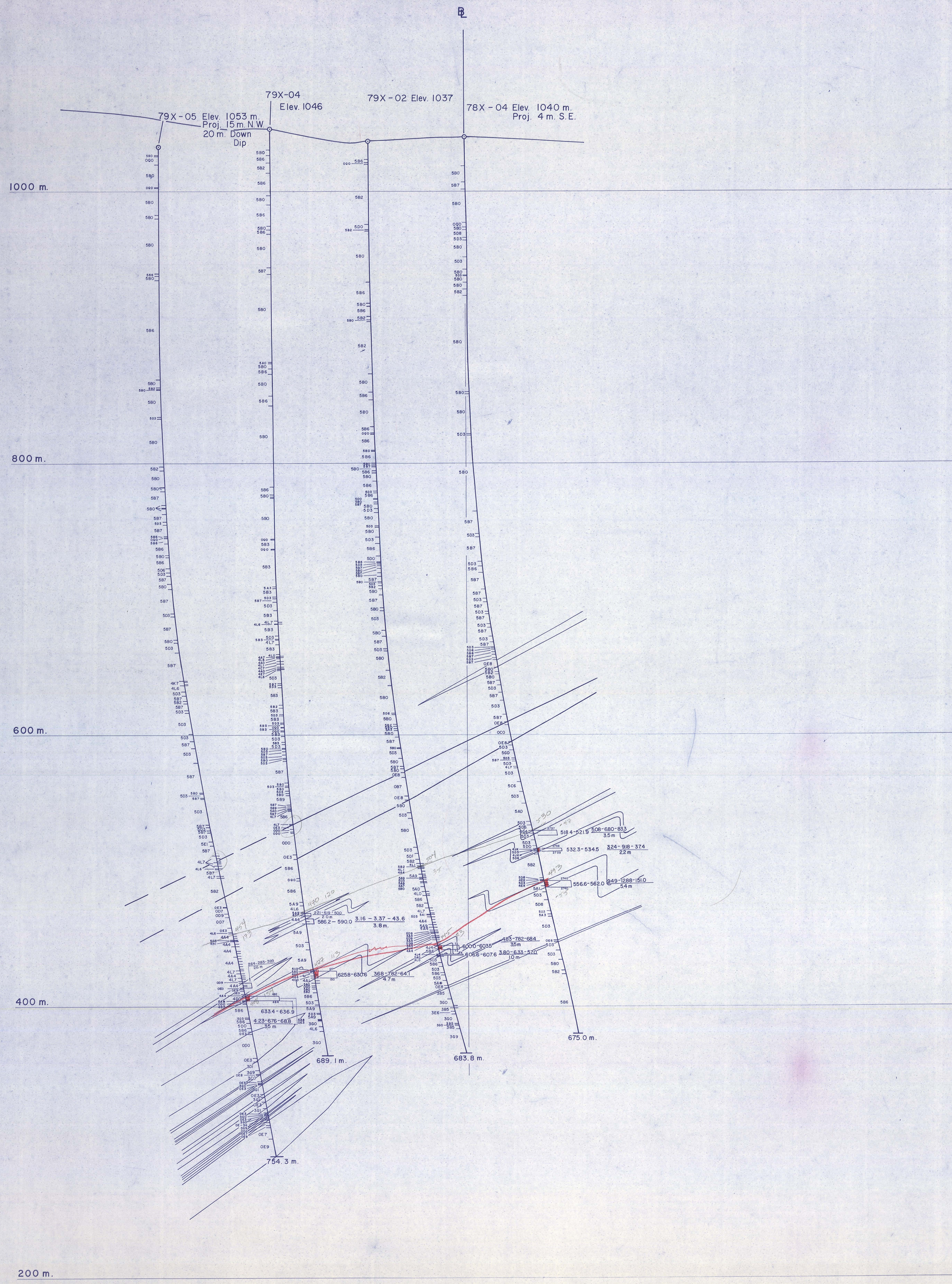
DY DEPOSIT VERTICAL CROSS SECTION 19+50E SCALE 1:1,000
