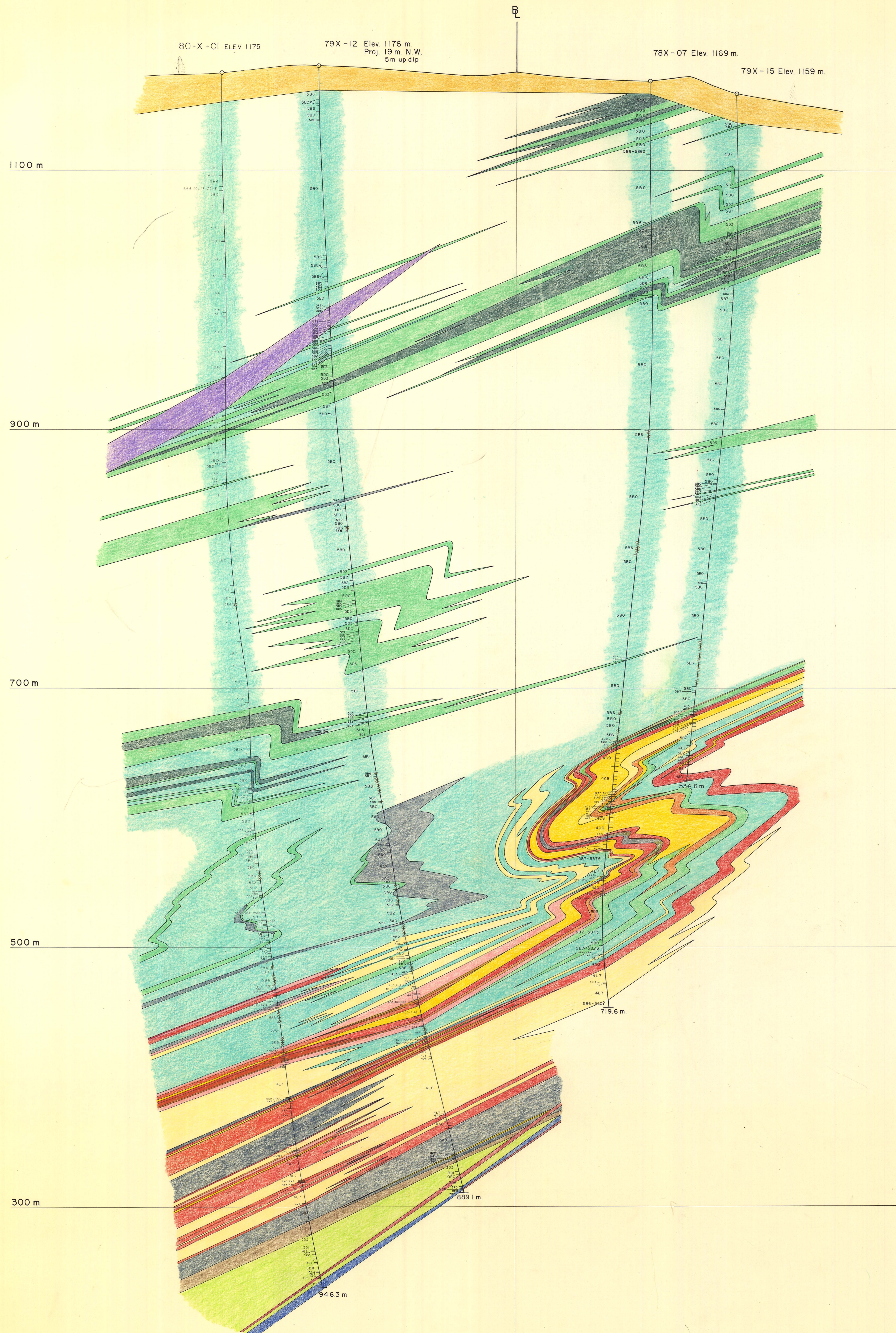
DY DEPOSIT VERTICAL CROSS SECTION 12 + 00E 007951 SCALE 1:1,000
