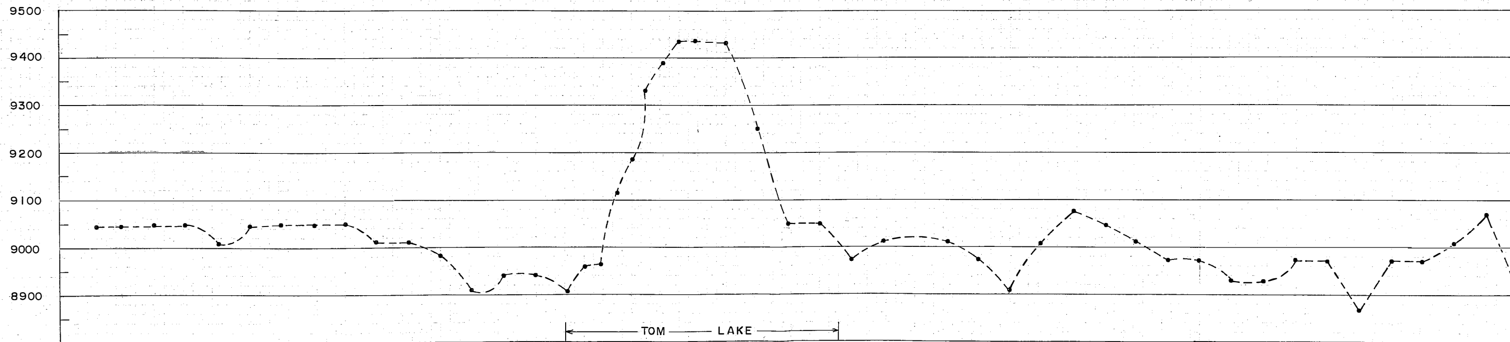
DAVIE GROUP (West half) GROUND MAGNETIC PROFILE LINE 30 W
