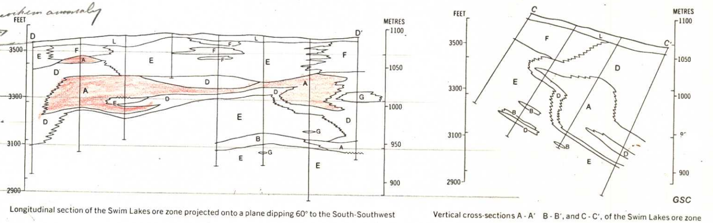
FIGURE 19. Cross-sections and map of the Swim Lakes deposit.
