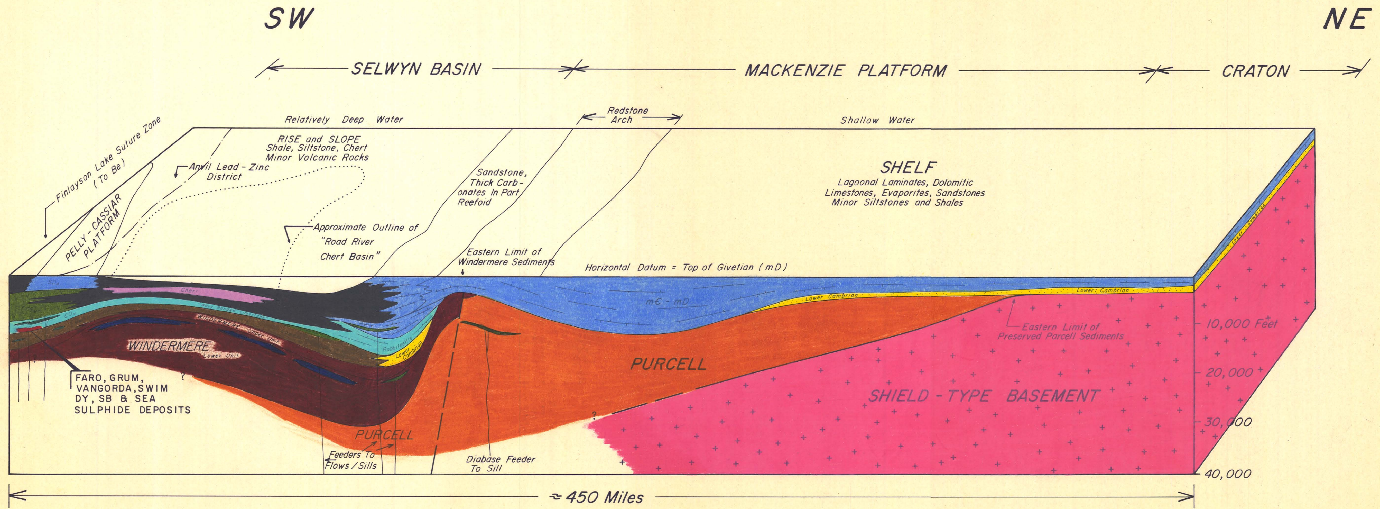
SCHEMATIC BLOCK DIAGRAM OF SELWYN BASIN / MACKENZIE PLATFORM (Upper Proterozoic / Lower Paleozoic) 009224
