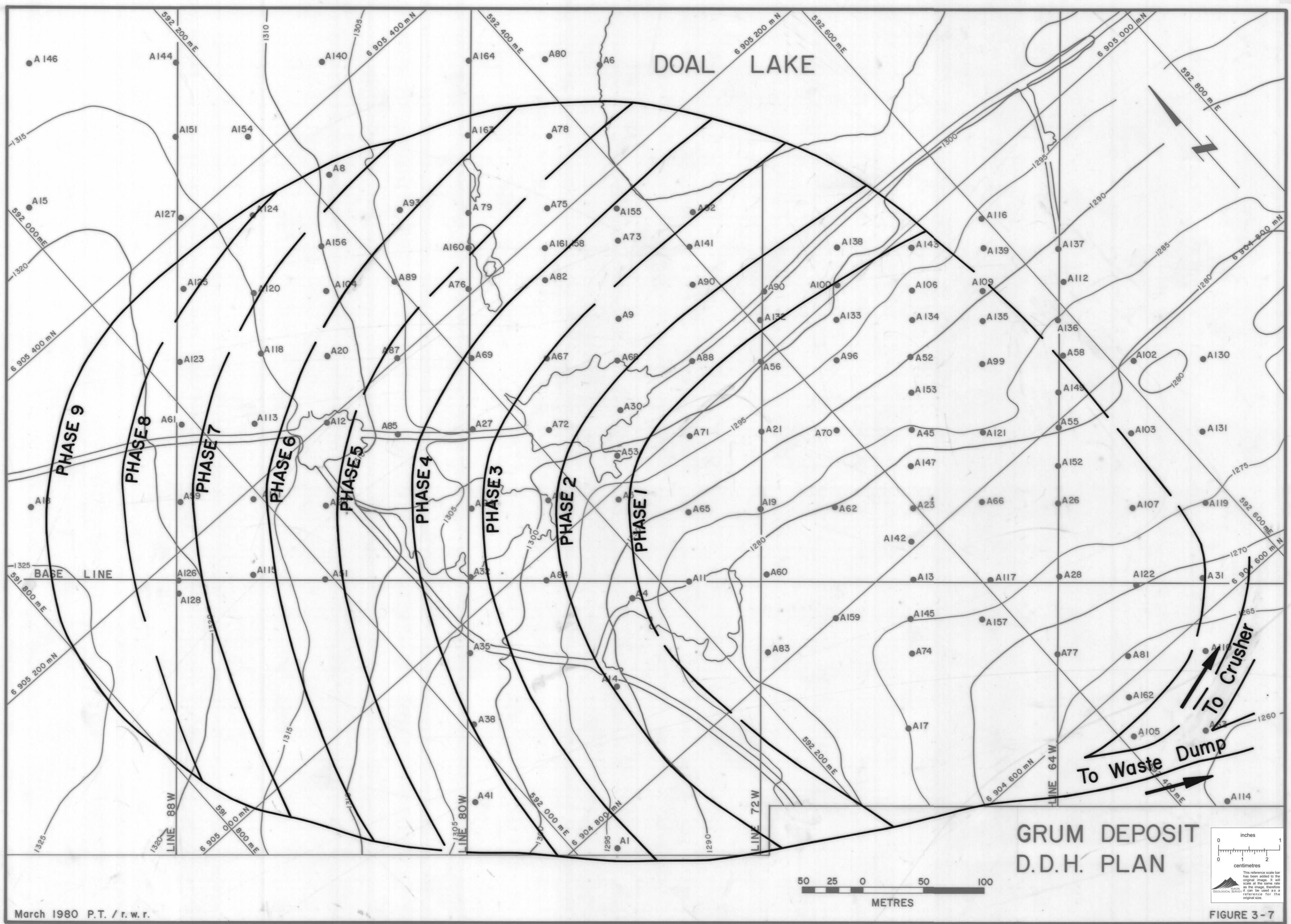
OPEN PIT OUTLINE
