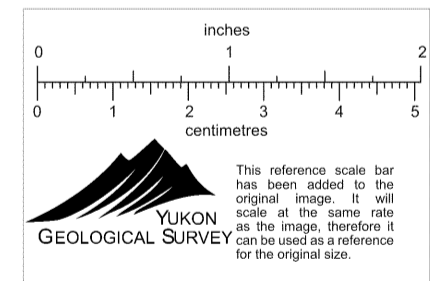
Figure 11 CYPRUS ANVIL MINING CORPORATION DANA HAL and HALO CLAIMS GRAPHIC LOG DDH 466 - 74 - 2 Scale: 1" = 100'
