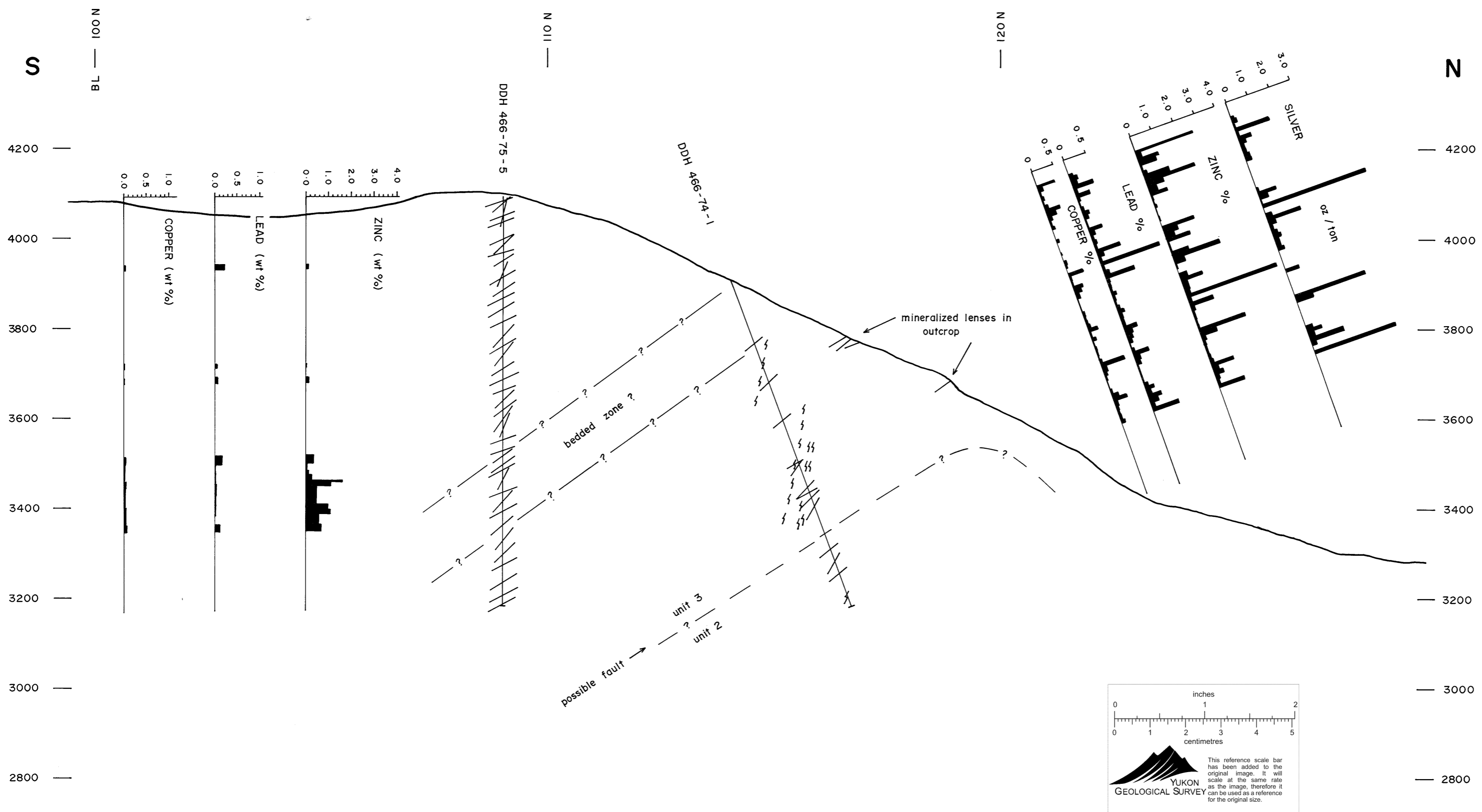
Figure 15 CYPRUS ANVIL MINING CORPORATION DANA and HALO CLAIMS SECTION ALONG L 36 E THROUGH DDH 466-74-1 & DDH 466-75-5 Horizontal & Vertical Scale: 1"=200'
