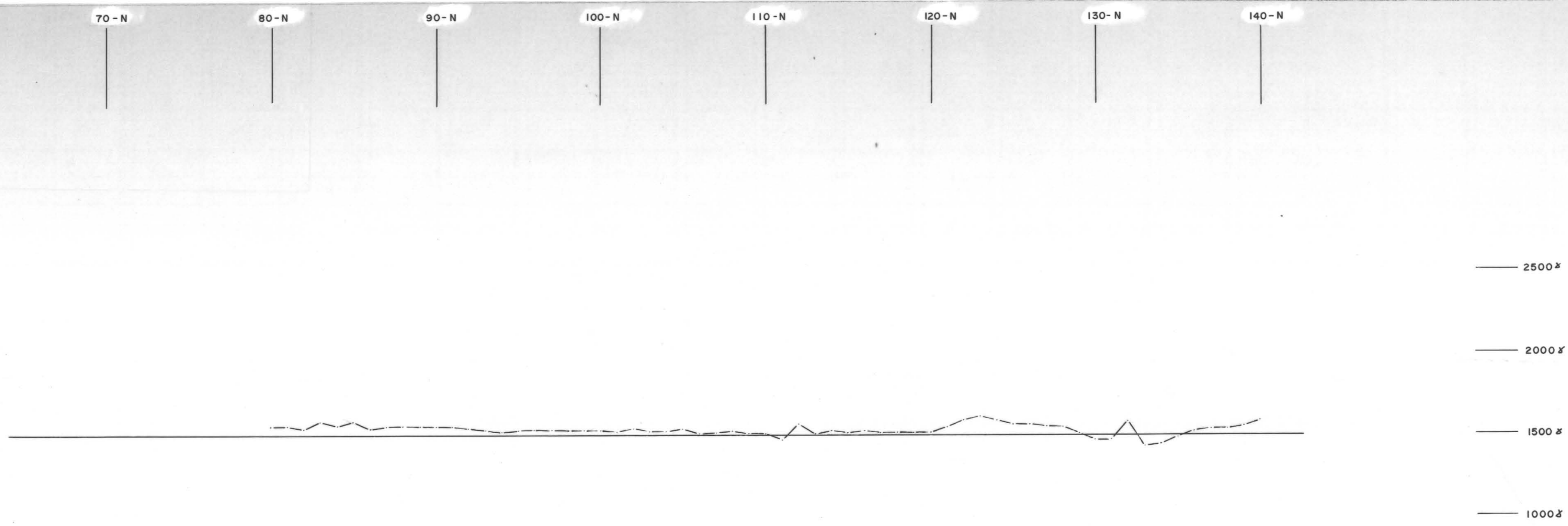
Profile of relative vertical intensity of magnetic field
