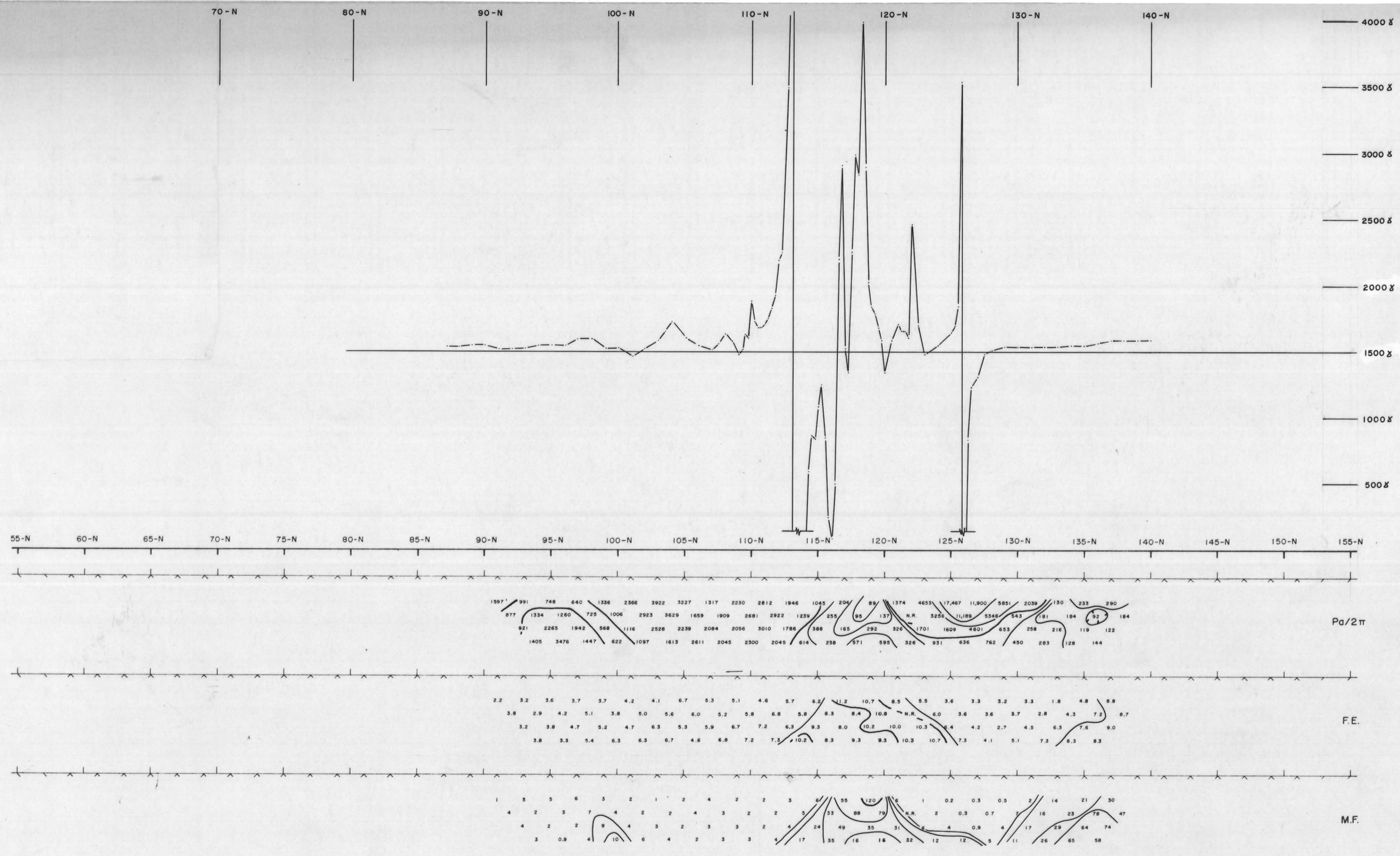
Profile of relative vertical intensity of magnetic field
