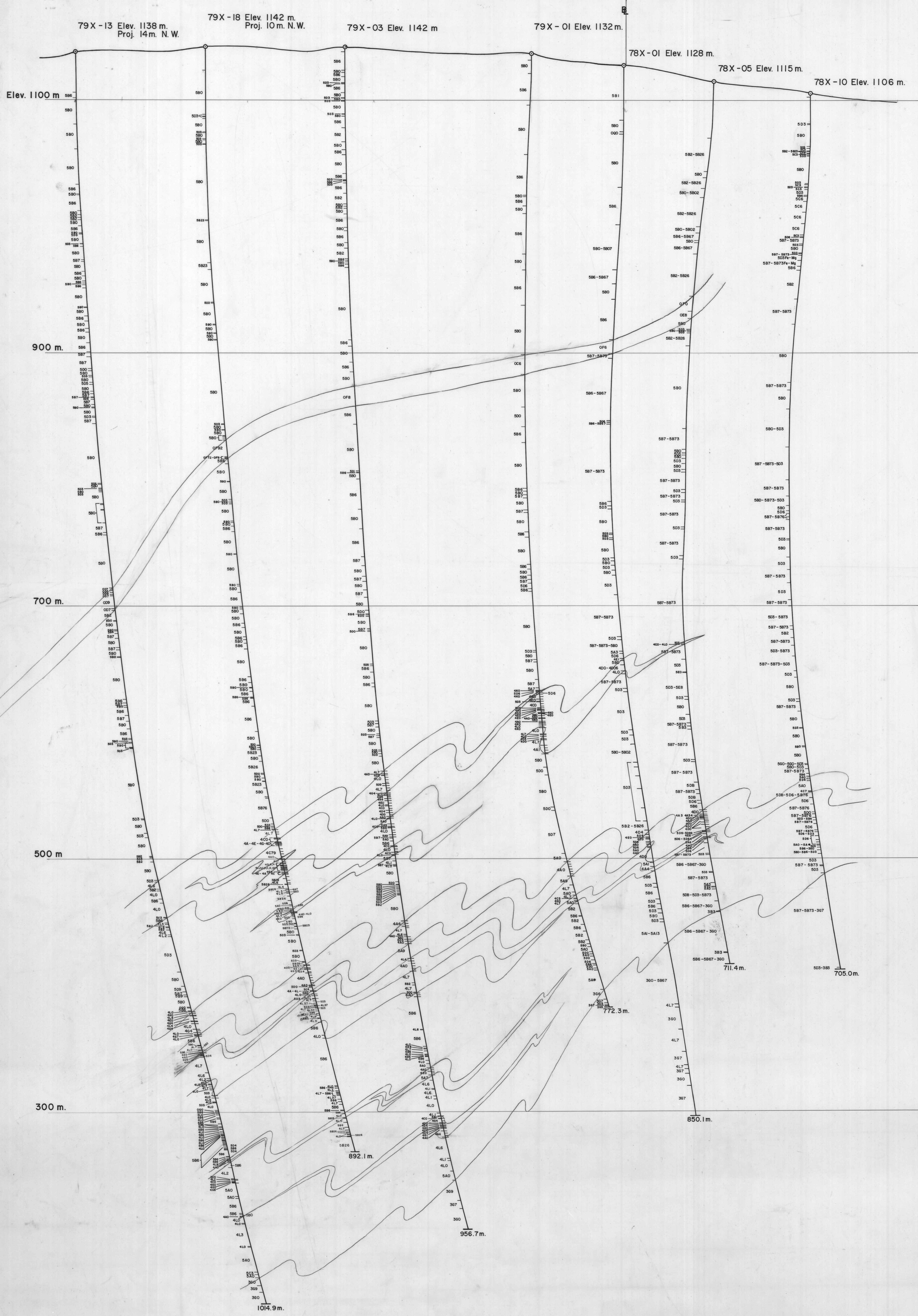
DY DEPOSIT VERTICAL CROSS SECTION 15+00 E SCALE 1:1,000
