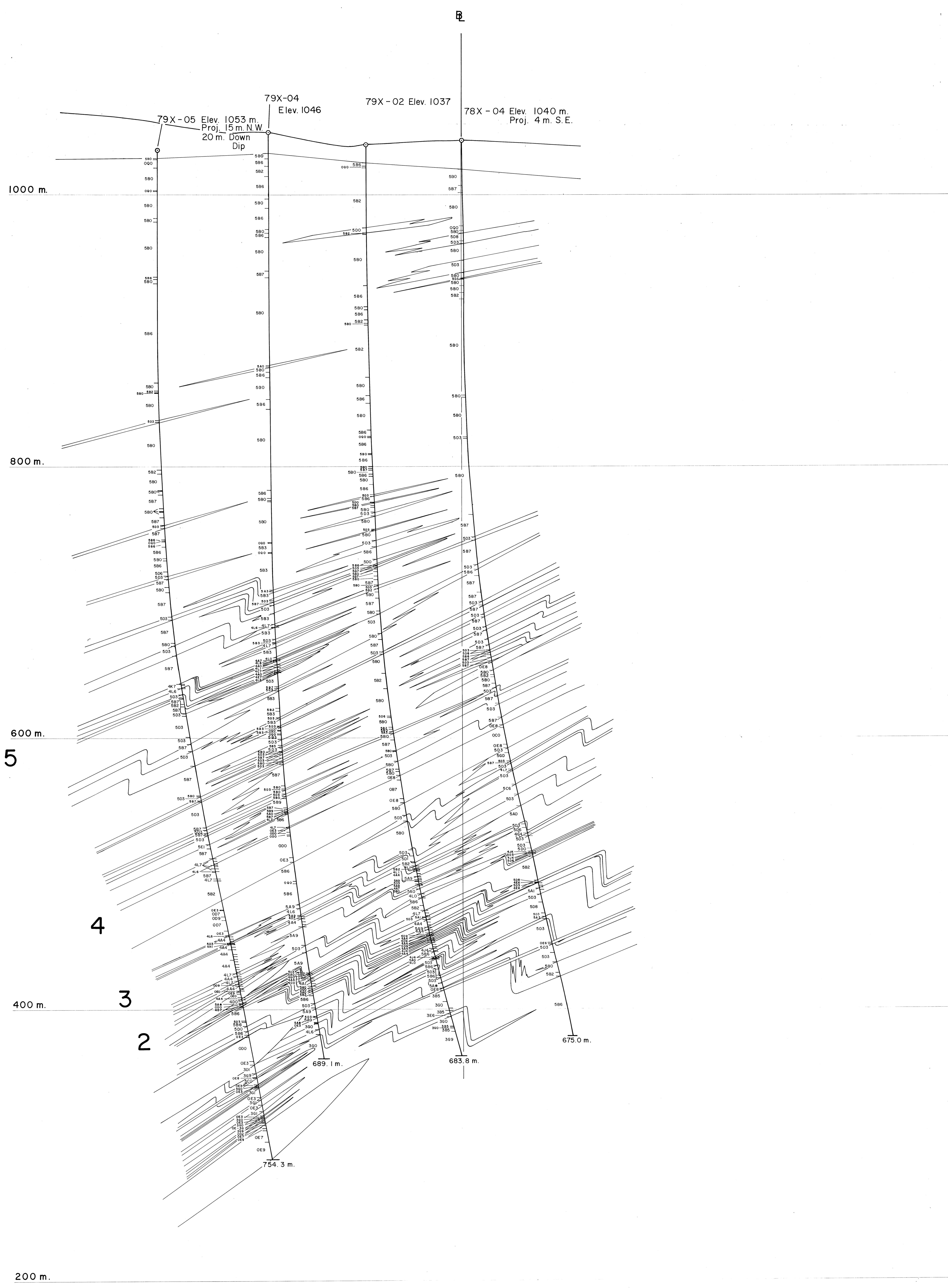
DY DEPOSIT VERTICAL CROSS SECTION 19+50E SCALE 1:1,000 19-3-80
