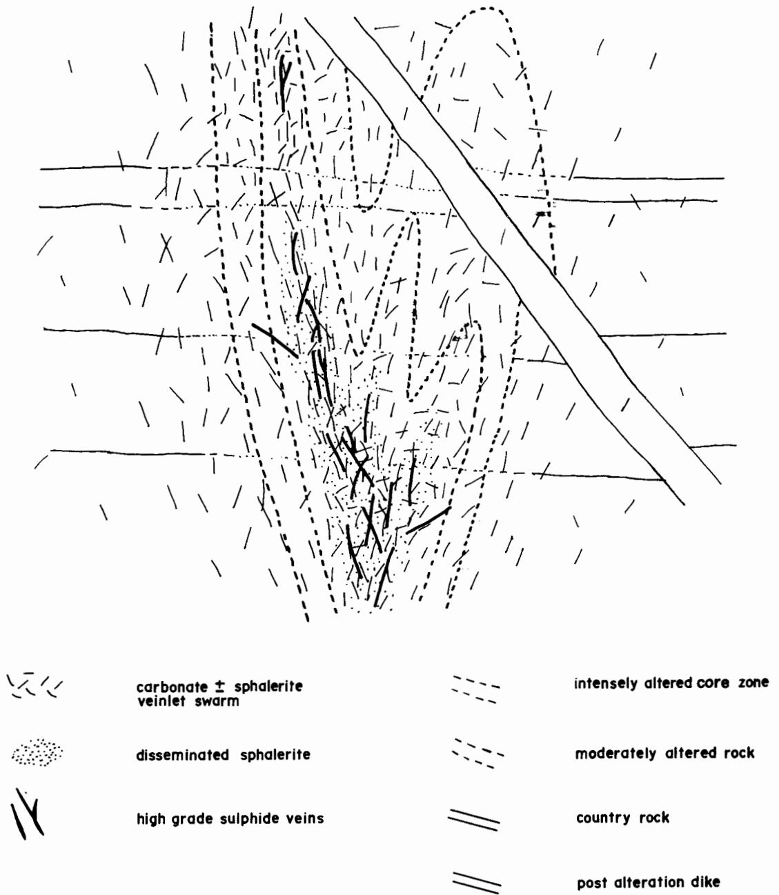
Figure 42 Diagrammatic cross section of the proposed type of mineralization on KD. hill before deformation and metamorphism.
