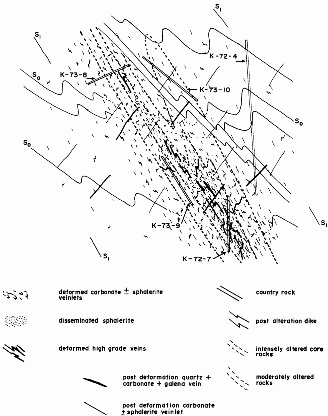
Figure 43. Diagrammatic section through model of KD hill mineralization showing some effects of deformation. Migration into low pressure areas is not shown and it is not known if this process has occurred on a large scale. Various hypothetical drill intersections show what parts of such a deposit might have been encountered by drill holes. The available evidence is not adequate to apply this model to a reliable true section through the KD hill.
