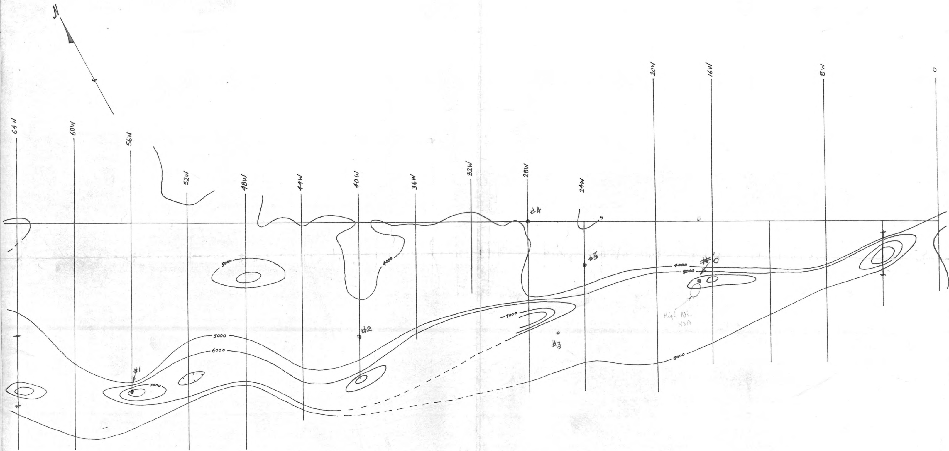
MAGNETIC CONTOURS OVER PART OF THE DICKSON CREEK NICKEL PROPERTY SCALE : 400 ft. to the inch CONTOUR INTERVAL : 1000 ♂
