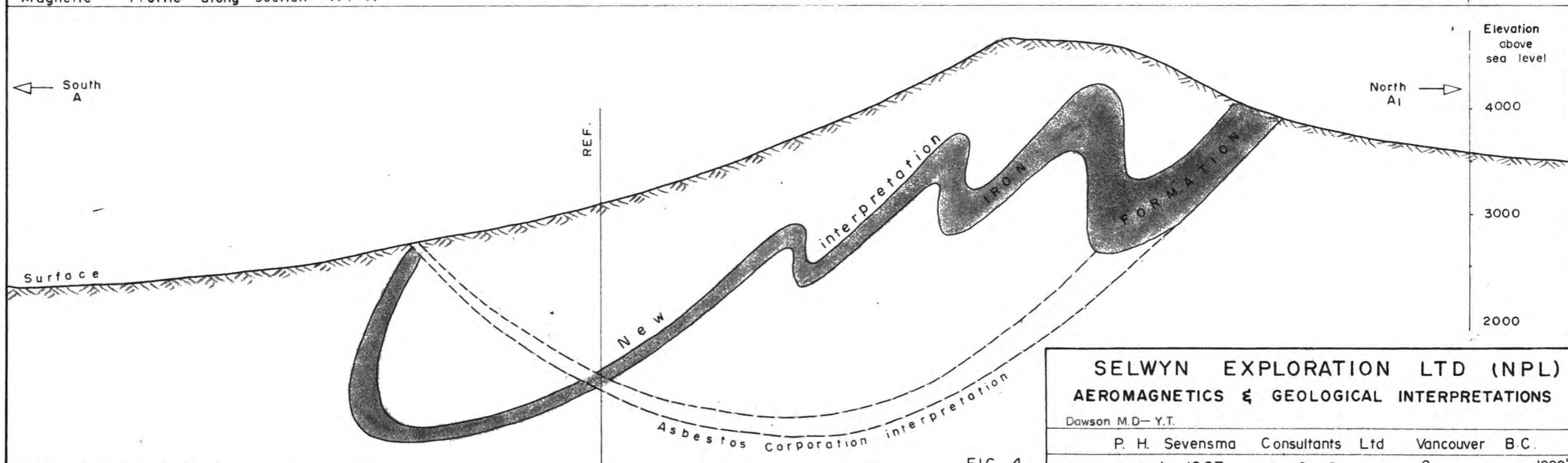
Ideal Geological Section A-A
