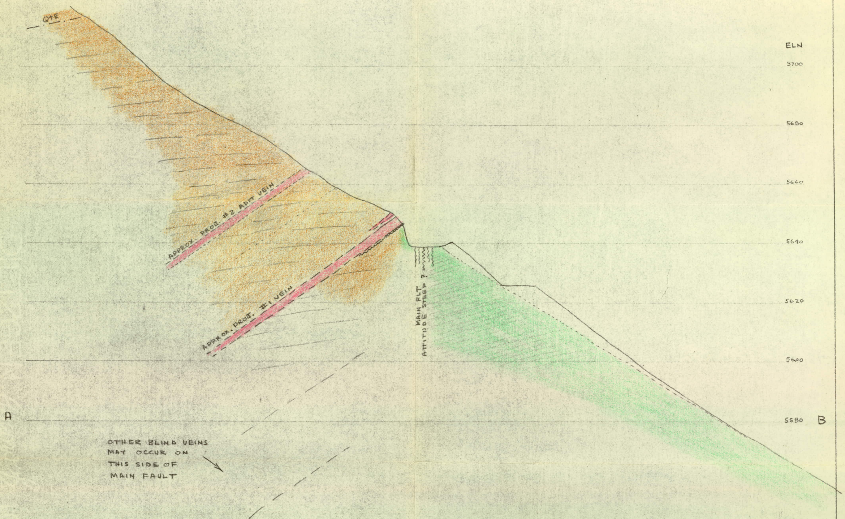
SKETCH SECTION A-B KEY 3A SHOWING KETZKEY SILVER MINES SCALE 1 IN. = 20 FT. A.E.AHO SEPT 15/61
