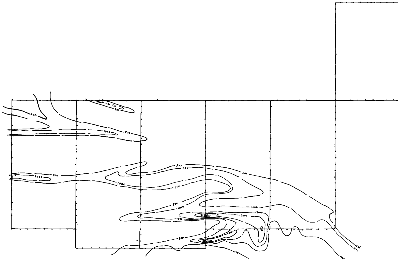
JAKE LAKE SOIL SAMPLE GRID ZN CONTOURS
