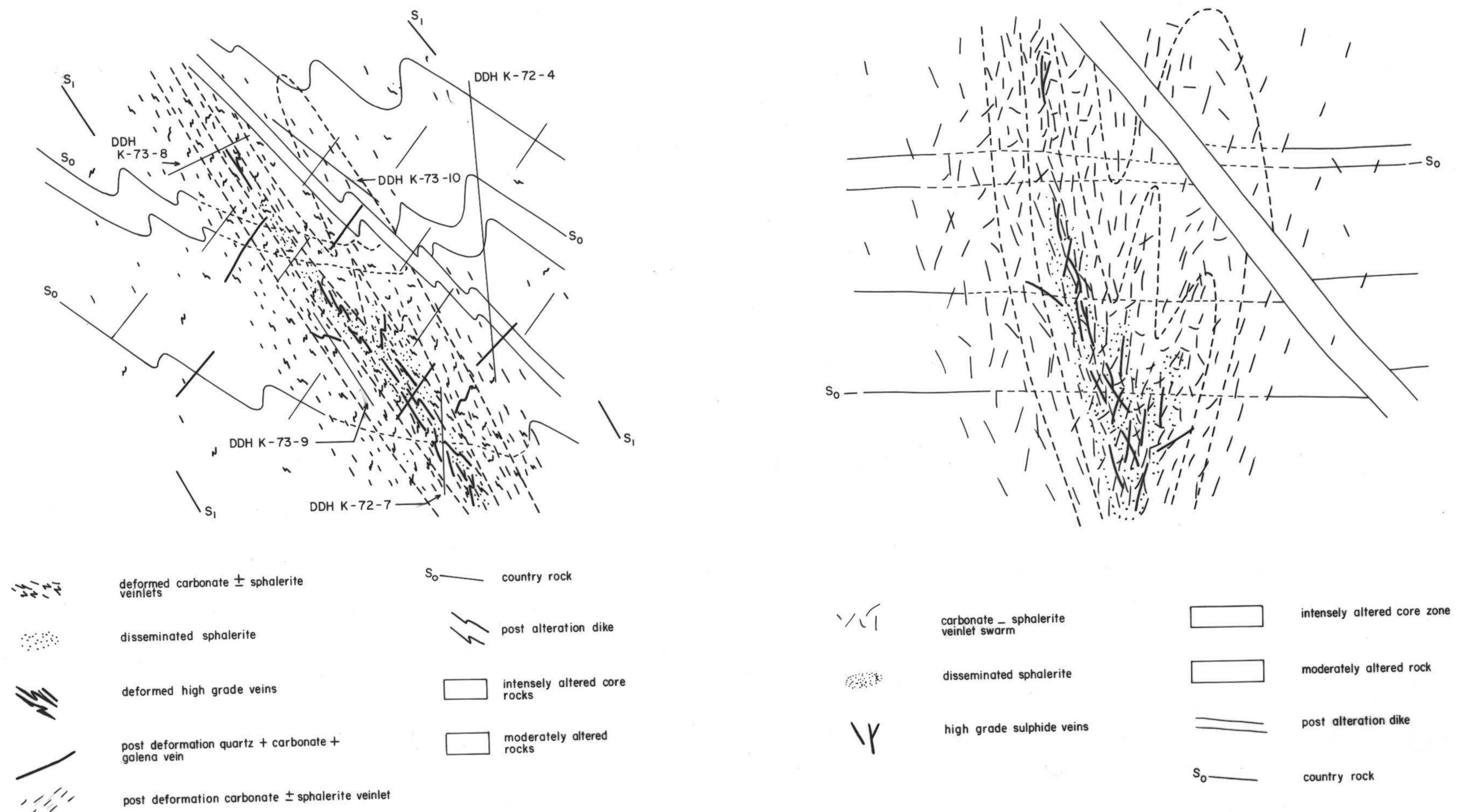
Schematic Cross Section Through Restored Idealized KD Deposit
