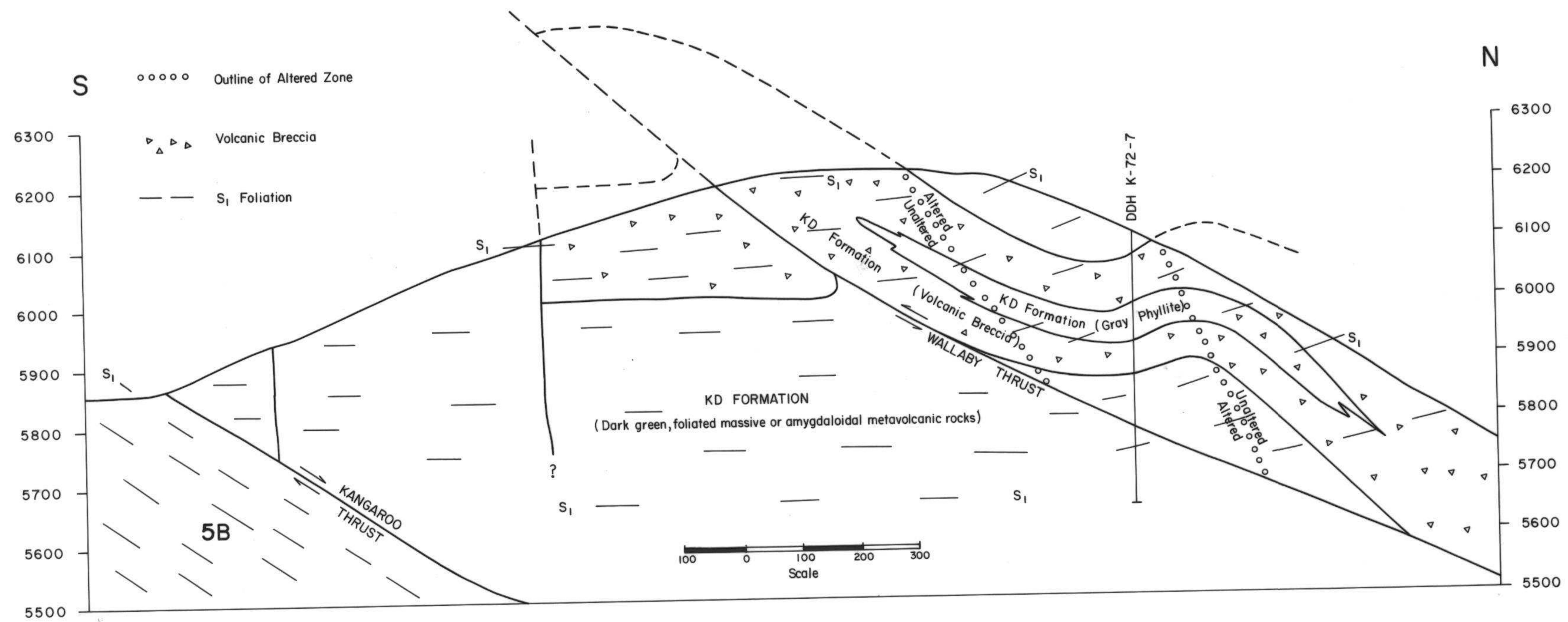
Representative Cross Section Through KD Deposit
