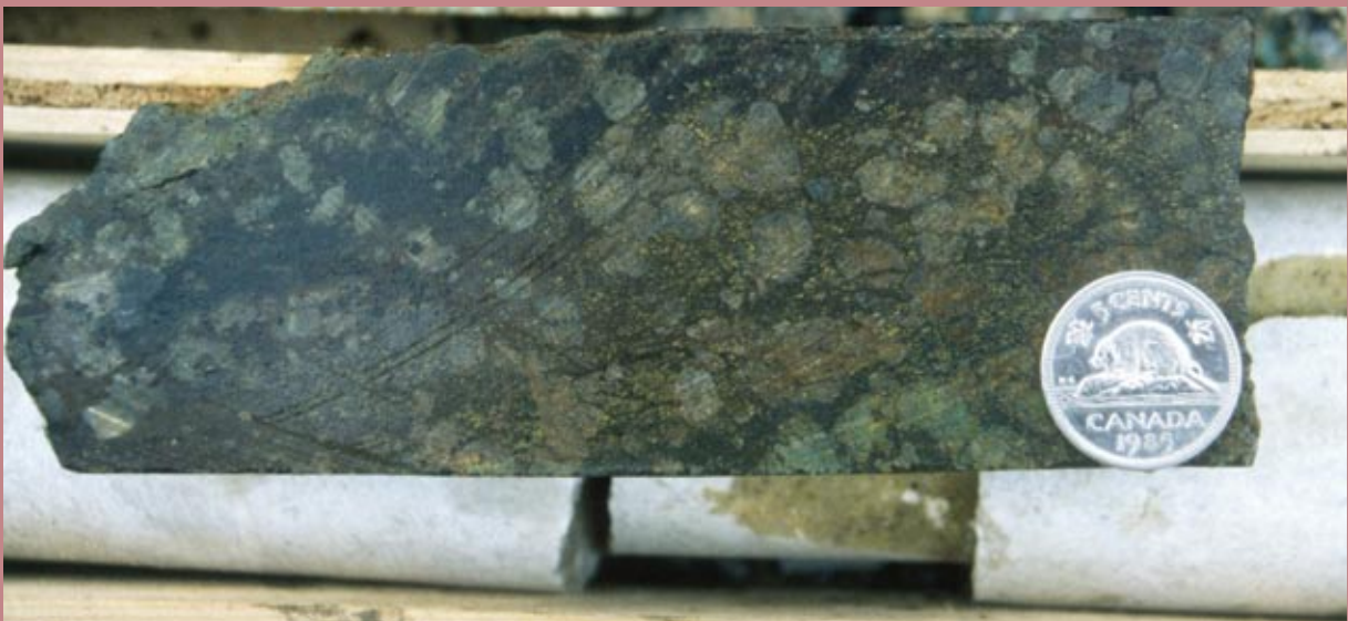
Magnetite, garnet, chalcopryite and bornite in core from a new copper skarn discovery, the Hat claims, near the past producing War Eagle deposit in the Whitehorse Copper Belt.
